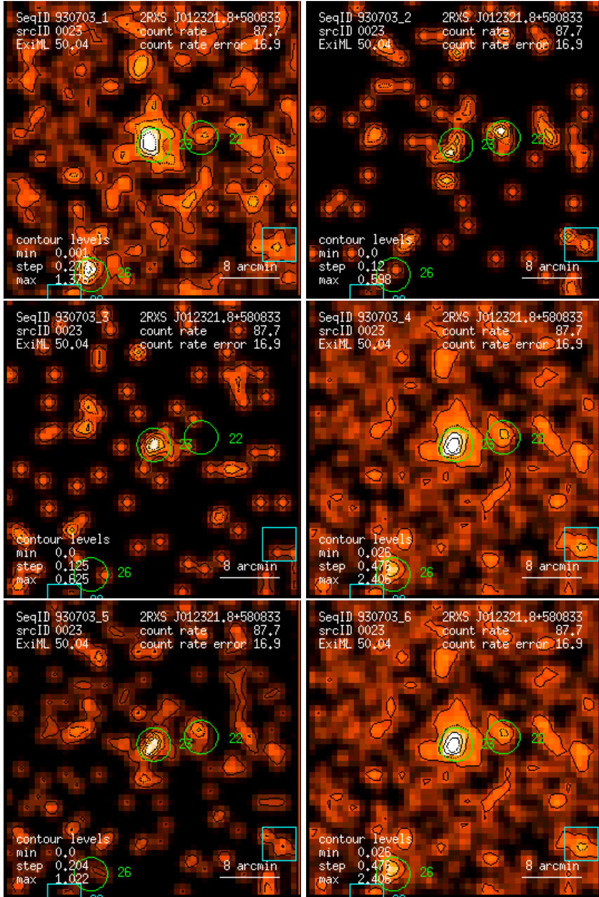
Figure 23: RASS 930703: detection 0023: band rate images, Gaussian filter: (1) PSPC channels 11 – 41, (2) 52 – 90, (3) 91 – 201, (4) 11 – 235, (5) 52 – 201, (6) 11 – 201. Broad band rates in counts/ks. Band rate contour levels in counts/ks/arcmin 2 .
