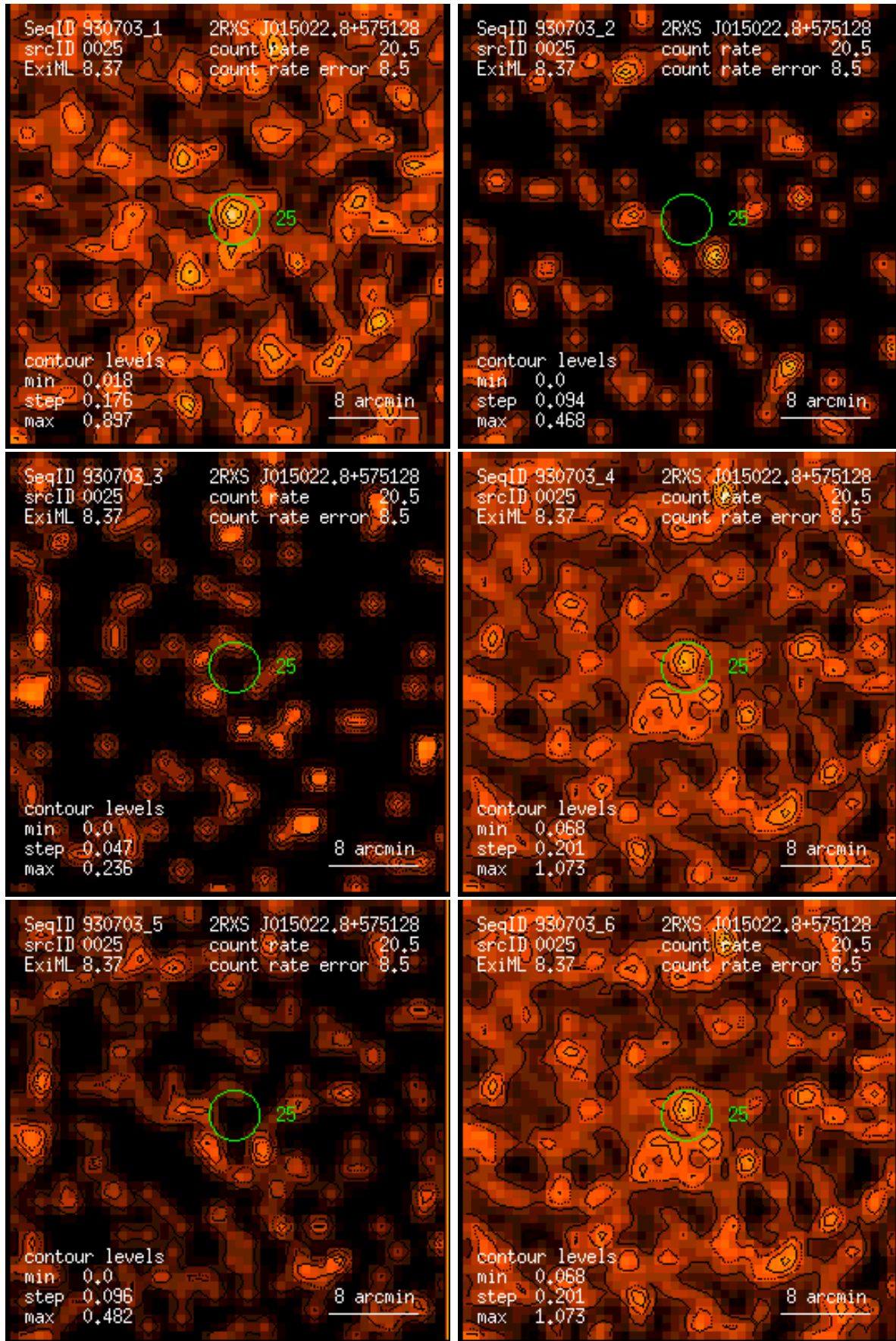
Figure 25: RASS 930703: detection 0025: band rate images, Gaussian filter: (1) PSPC channels 11 – 41, (2) 52 – 90, (3) 91 – 201, (4) 11 – 235, (5) 52 – 201, (6) 11 – 201. Broad band rates in counts/ks. Band rate contour levels in counts/ks/arcmin 2 .
