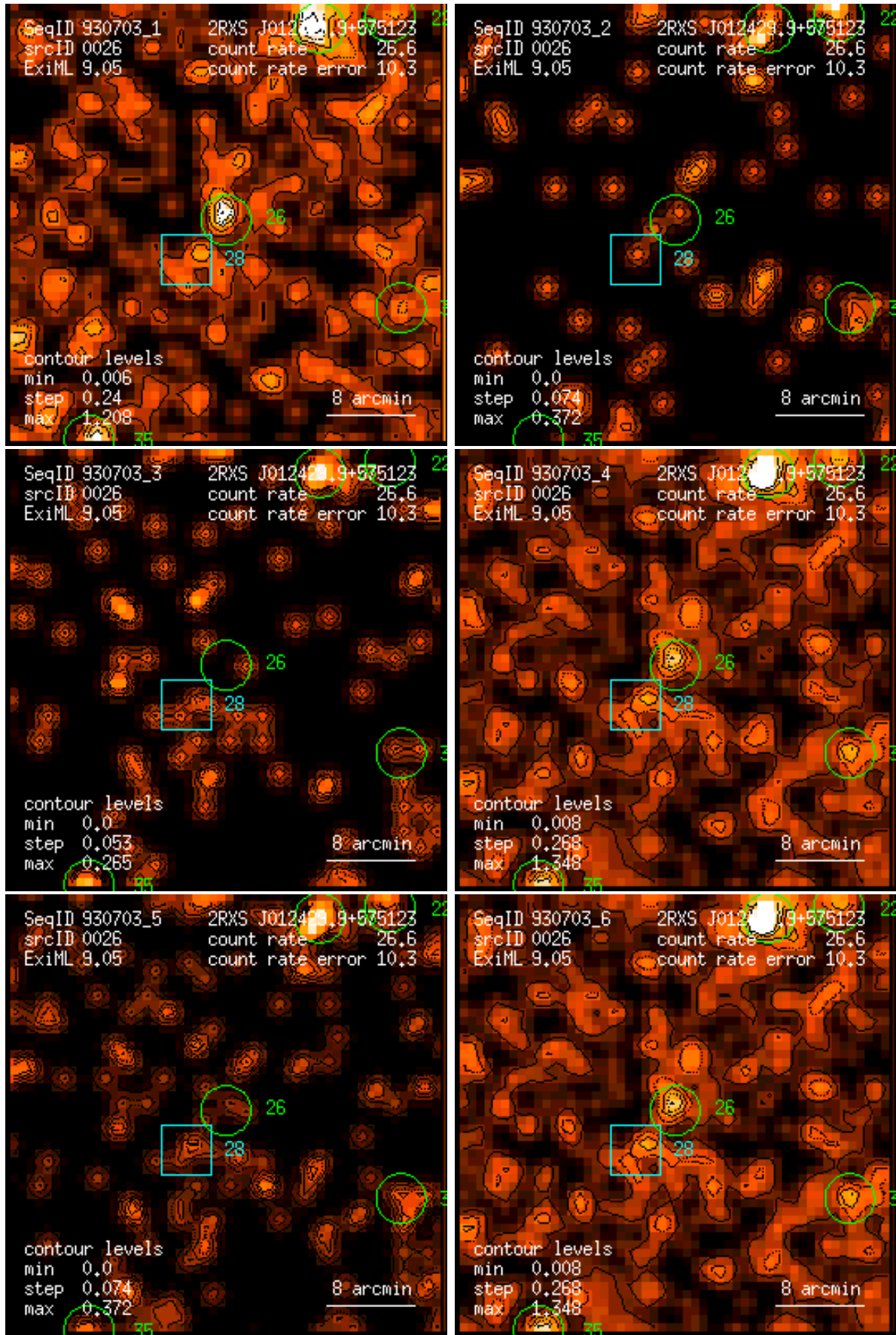
Figure 26: RASS 930703: detection 0026: band rate images, Gaussian filter: (1) PSPC channels 11 – 41, (2) 52 – 90, (3) 91 – 201, (4) 11 – 235, (5) 52 – 201, (6) 11 – 201. Broad band rates in counts/ks. Band rate contour levels in counts/ks/arcmin 2 .
