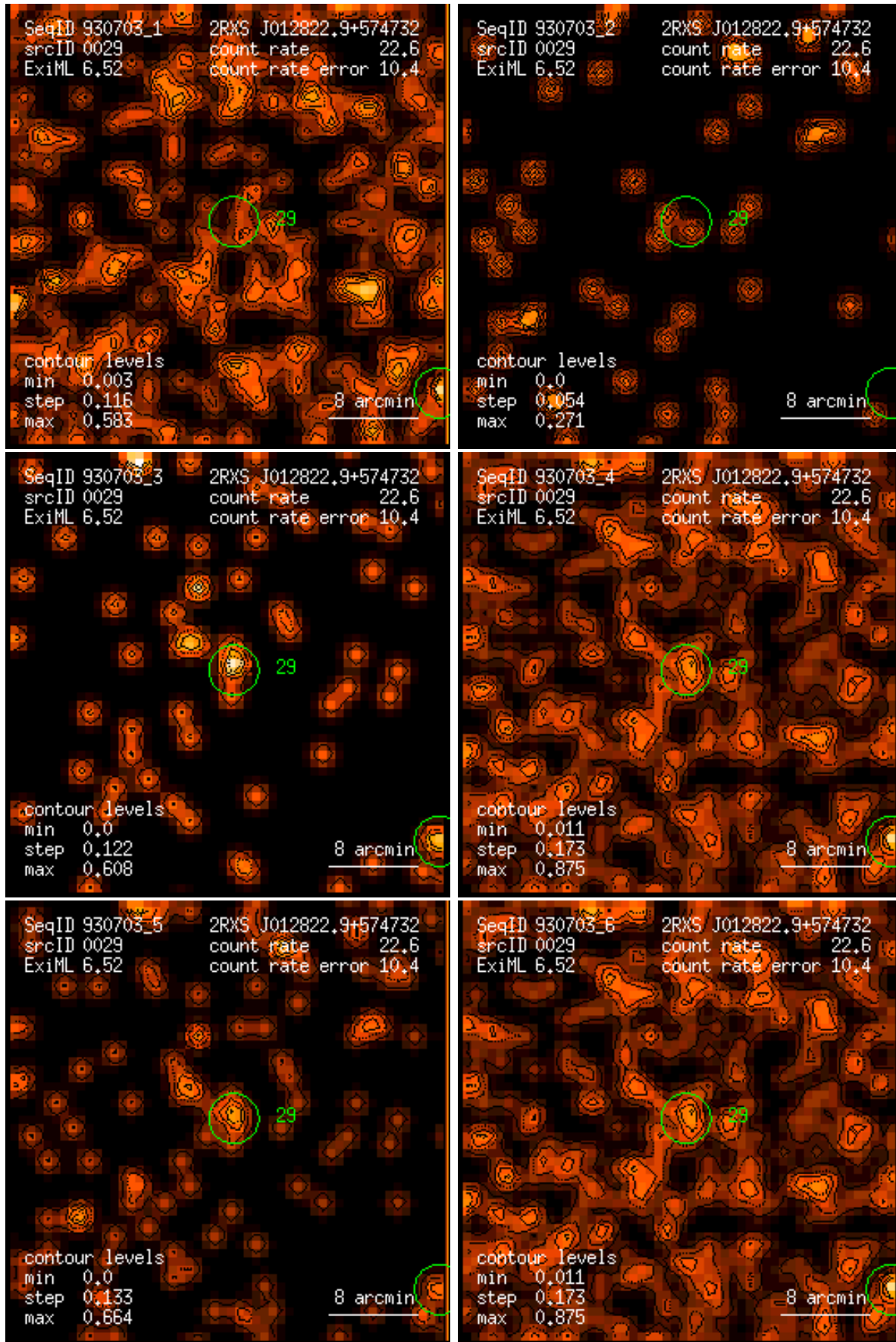
Figure 29: RASS 930703: detection 0029: band rate images, Gaussian filter: (1) PSPC channels 11 – 41, (2) 52 – 90, (3) 91 – 201, (4) 11 – 235, (5) 52 – 201, (6) 11 – 201. Broad band rates in counts/ks. Band rate contour levels in counts/ks/arcmin 2 .
