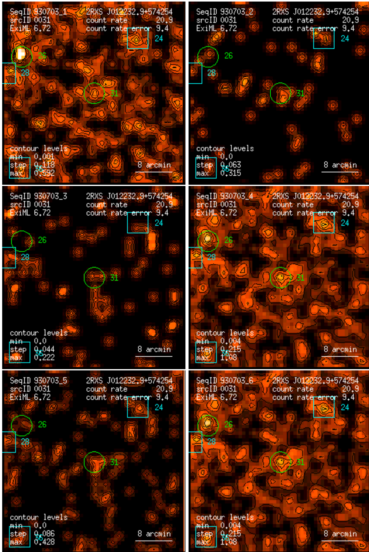
Figure 31: RASS 930703: detection 0031: band rate images, Gaussian filter: (1) PSPC channels 11 – 41, (2) 52 – 90, (3) 91 – 201, (4) 11 – 235, (5) 52 – 201, (6) 11 – 201. Broad band rates in counts/ks. Band rate contour levels in counts/ks/arcmin 2 .
