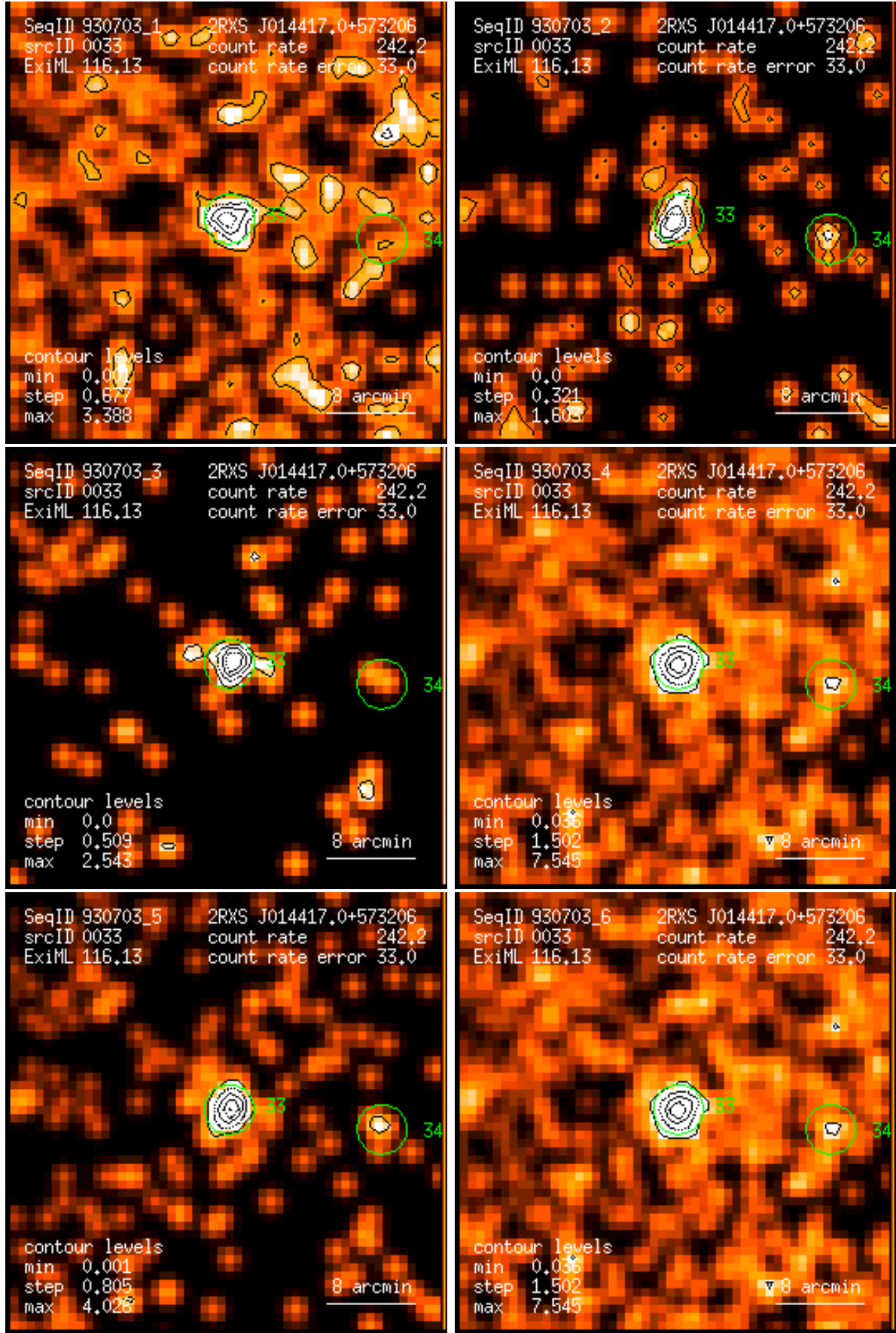
Figure 33: RASS 930703: detection 0033: band rate images, Gaussian filter: (1) PSPC channels 11 – 41, (2) 52 – 90, (3) 91 – 201, (4) 11 – 235, (5) 52 – 201, (6) 11 – 201. Broad band rates in counts/ks. Band rate contour levels in counts/ks/arcmin 2 .
