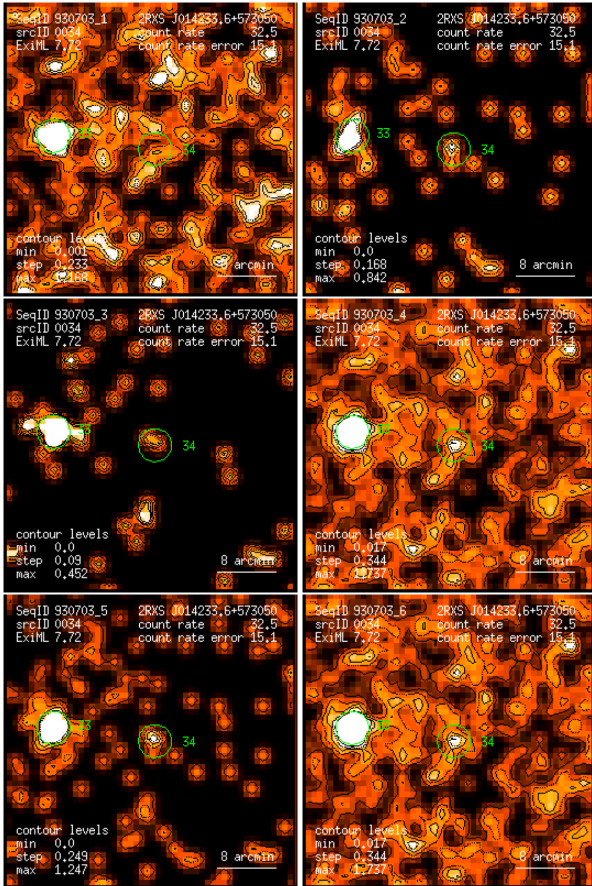
Figure 34: RASS 930703: detection 0034: band rate images, Gaussian filter: (1) PSPC channels 11 – 41, (2) 52 – 90, (3) 91 – 201, (4) 11 – 235, (5) 52 – 201, (6) 11 – 201. Broad band rates in counts/ks. Band rate contour levels in counts/ks/arcmin 2 .
