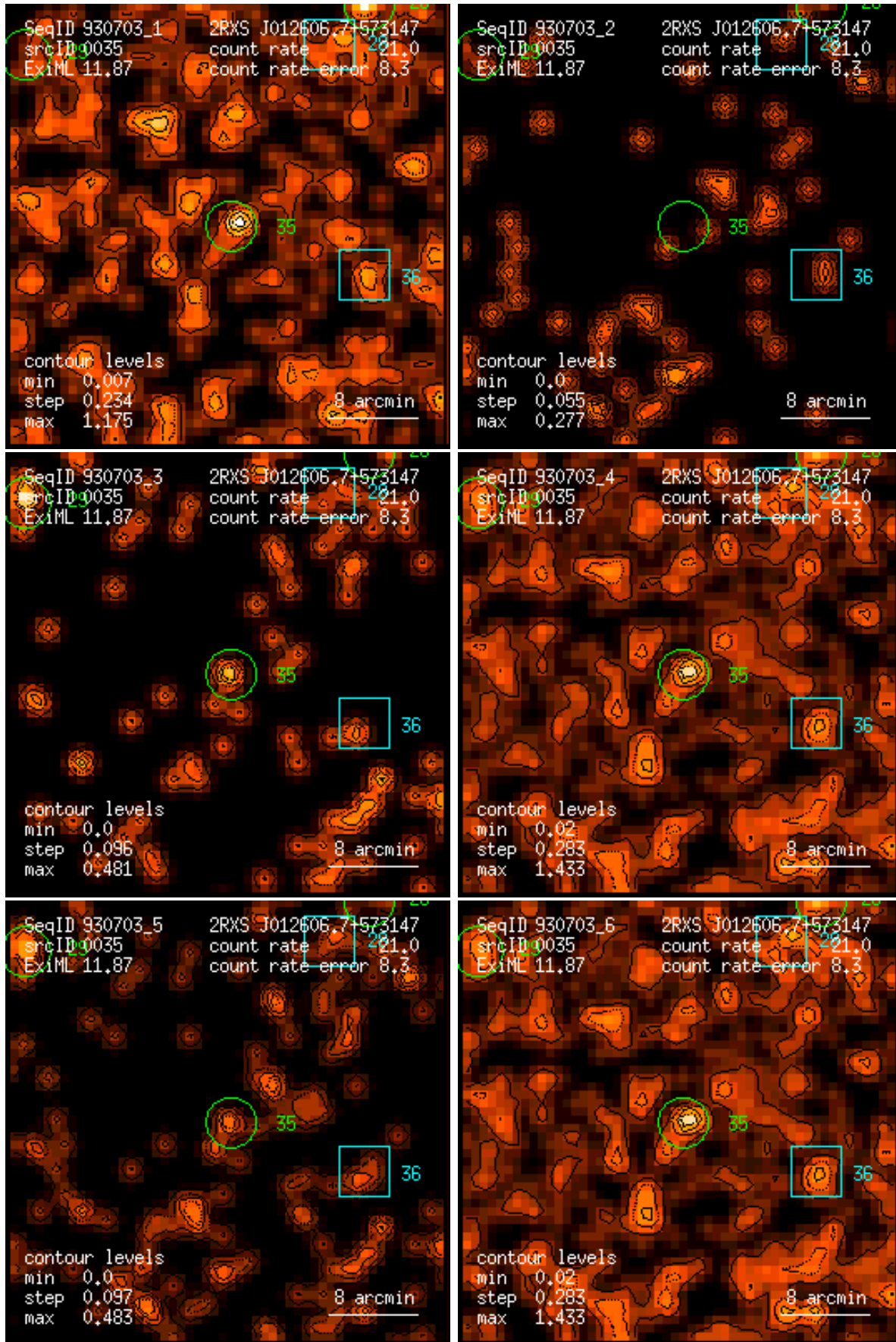
Figure 35: RASS 930703: detection 0035: band rate images, Gaussian filter: (1) PSPC channels 11 – 41, (2) 52 – 90, (3) 91 – 201, (4) 11 – 235, (5) 52 – 201, (6) 11 – 201. Broad band rates in counts/ks. Band rate contour levels in counts/ks/arcmin 2 .
