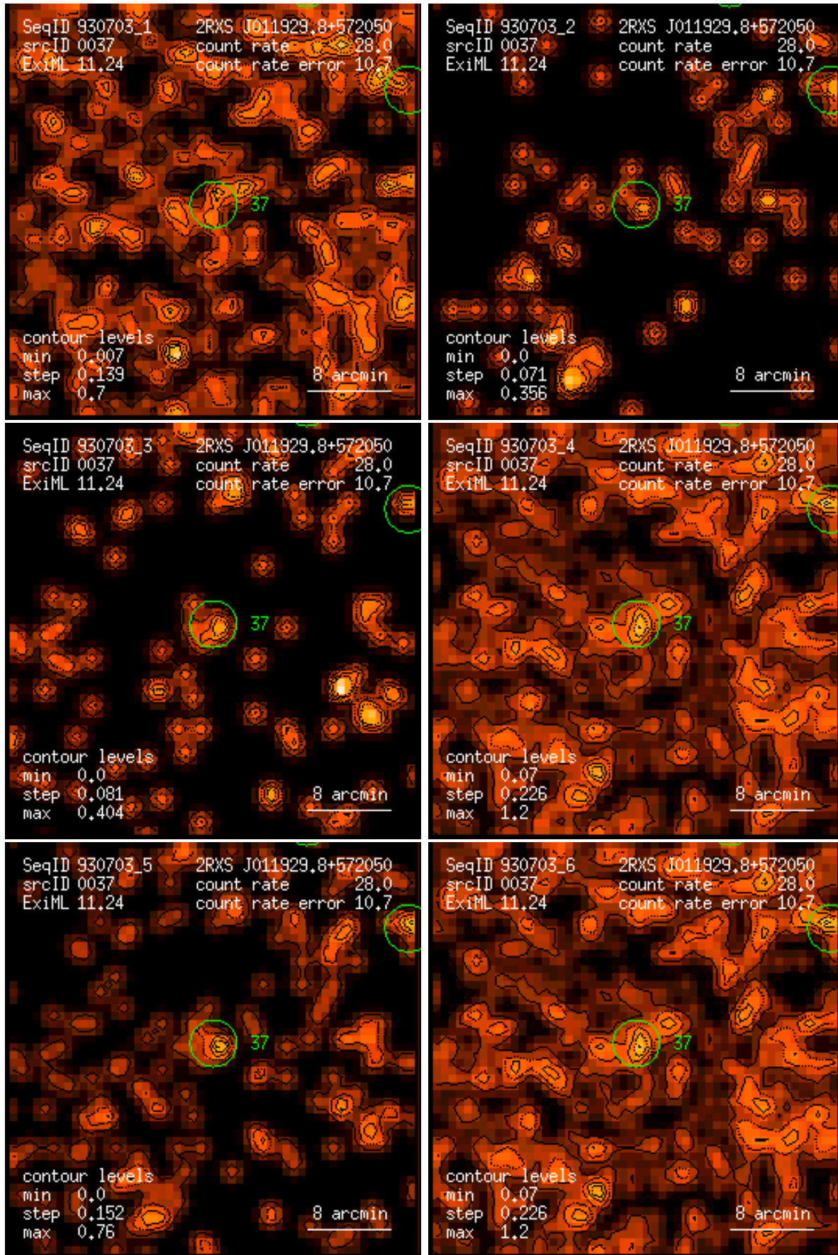
Figure 37: RASS 930703: detection 0037: band rate images, Gaussian filter: (1) PSPC channels 11 – 41, (2) 52 – 90, (3) 91 – 201, (4) 11 – 235, (5) 52 – 201, (6) 11 – 201. Broad band rates in counts/ks. Band rate contour levels in counts/ks/arcmin 2 .
