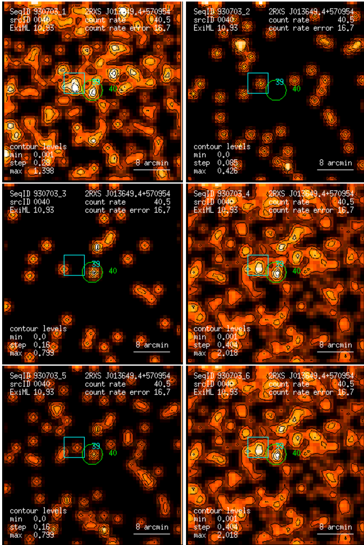
Figure 40: RASS 930703: detection 0040: band rate images, Gaussian filter: (1) PSPC channels 11 – 41, (2) 52 – 90, (3) 91 – 201, (4) 11 – 235, (5) 52 – 201, (6) 11 – 201. Broad band rates in counts/ks. Band rate contour levels in counts/ks/arcmin 2 .
