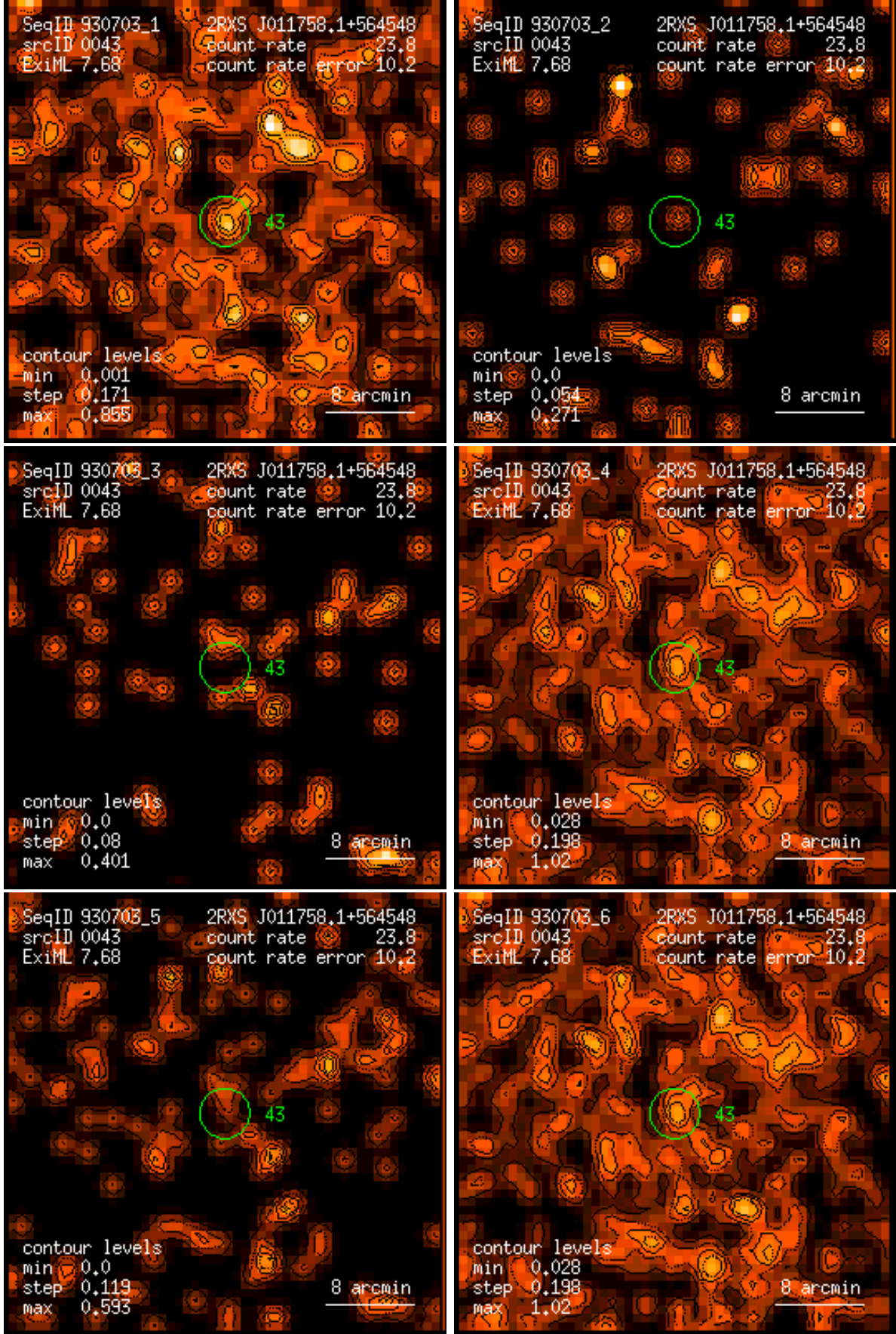
Figure 43: RASS 930703: detection 0043: band rate images, Gaussian filter: (1) PSPC channels 11 – 41, (2) 52 – 90, (3) 91 – 201, (4) 11 – 235, (5) 52 – 201, (6) 11 – 201. Broad band rates in counts/ks. Band rate contour levels in counts/ks/arcmin 2 .
