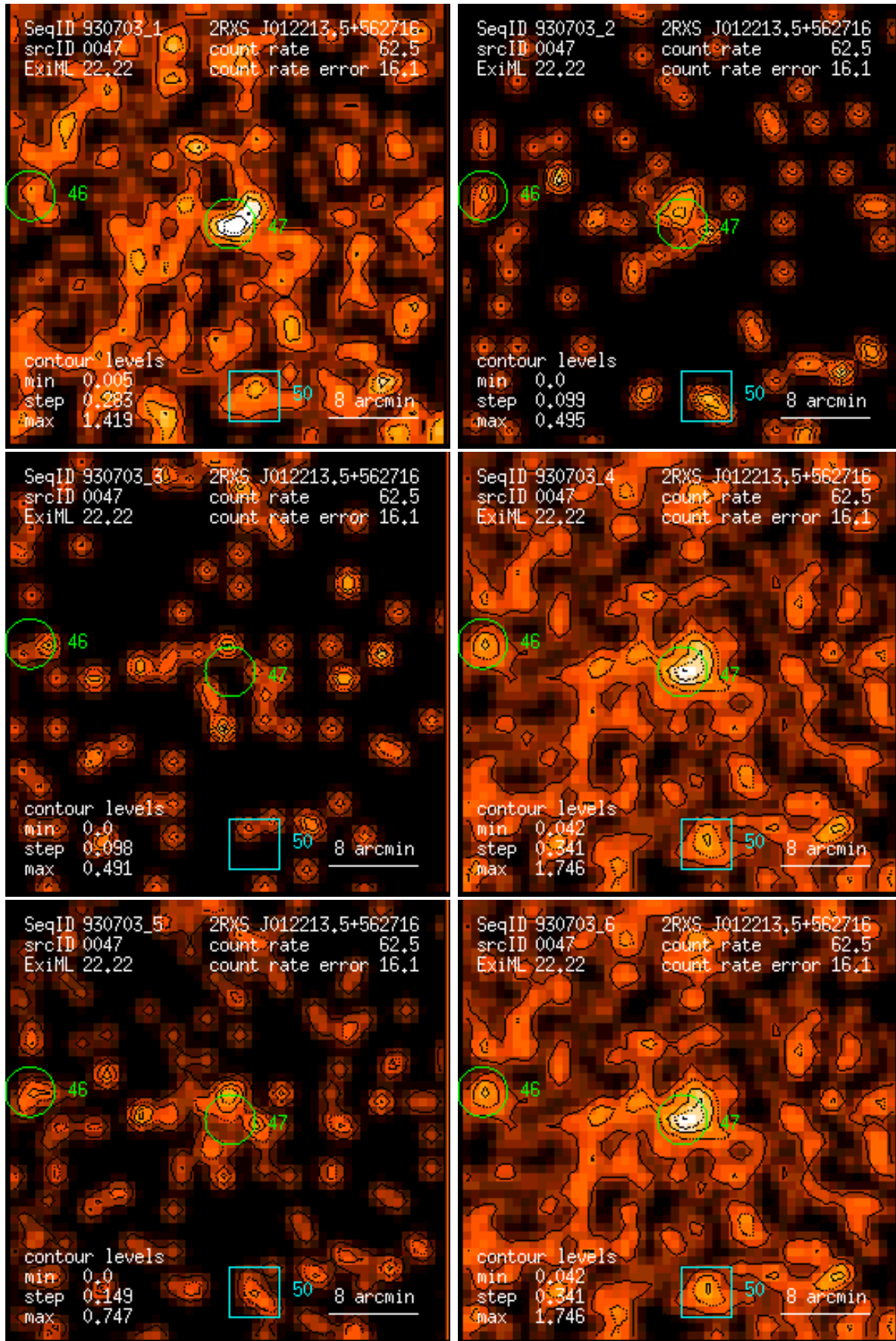
Figure 47: RASS 930703: detection 0047: band rate images, Gaussian filter: (1) PSPC channels 11 – 41, (2) 52 – 90, (3) 91 – 201, (4) 11 – 235, (5) 52 – 201, (6) 11 – 201. Broad band rates in counts/ks. Band rate contour levels in counts/ks/arcmin 2 .
