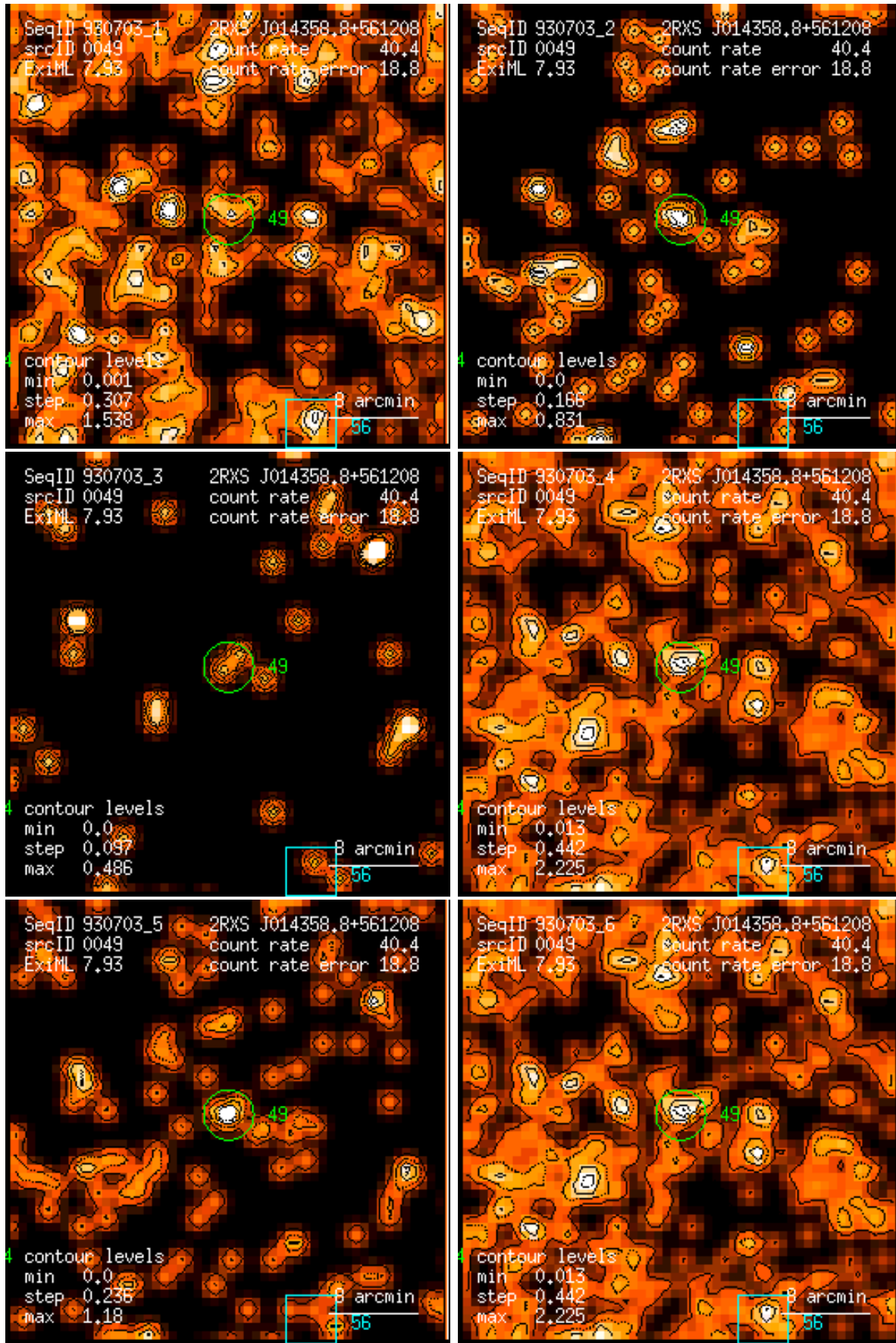
Figure 49: RASS 930703: detection 0049: band rate images, Gaussian filter: (1) PSPC channels 11 – 41, (2) 52 – 90, (3) 91 – 201, (4) 11 – 235, (5) 52 – 201, (6) 11 – 201. Broad band rates in counts/ks. Band rate contour levels in counts/ks/arcmin 2 .
