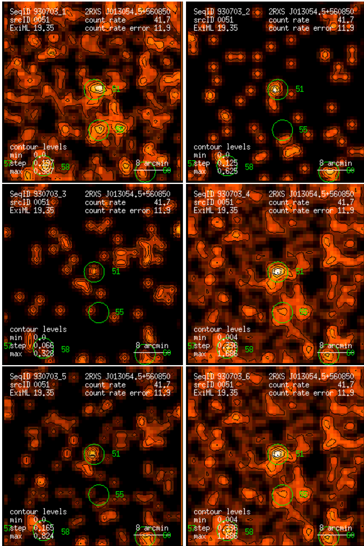
Figure 51: RASS 930703: detection 0051: band rate images, Gaussian filter: (1) PSPC channels 11 – 41, (2) 52 – 90, (3) 91 – 201, (4) 11 – 235, (5) 52 – 201, (6) 11 – 201. Broad band rates in counts/ks. Band rate contour levels in counts/ks/arcmin 2 .
