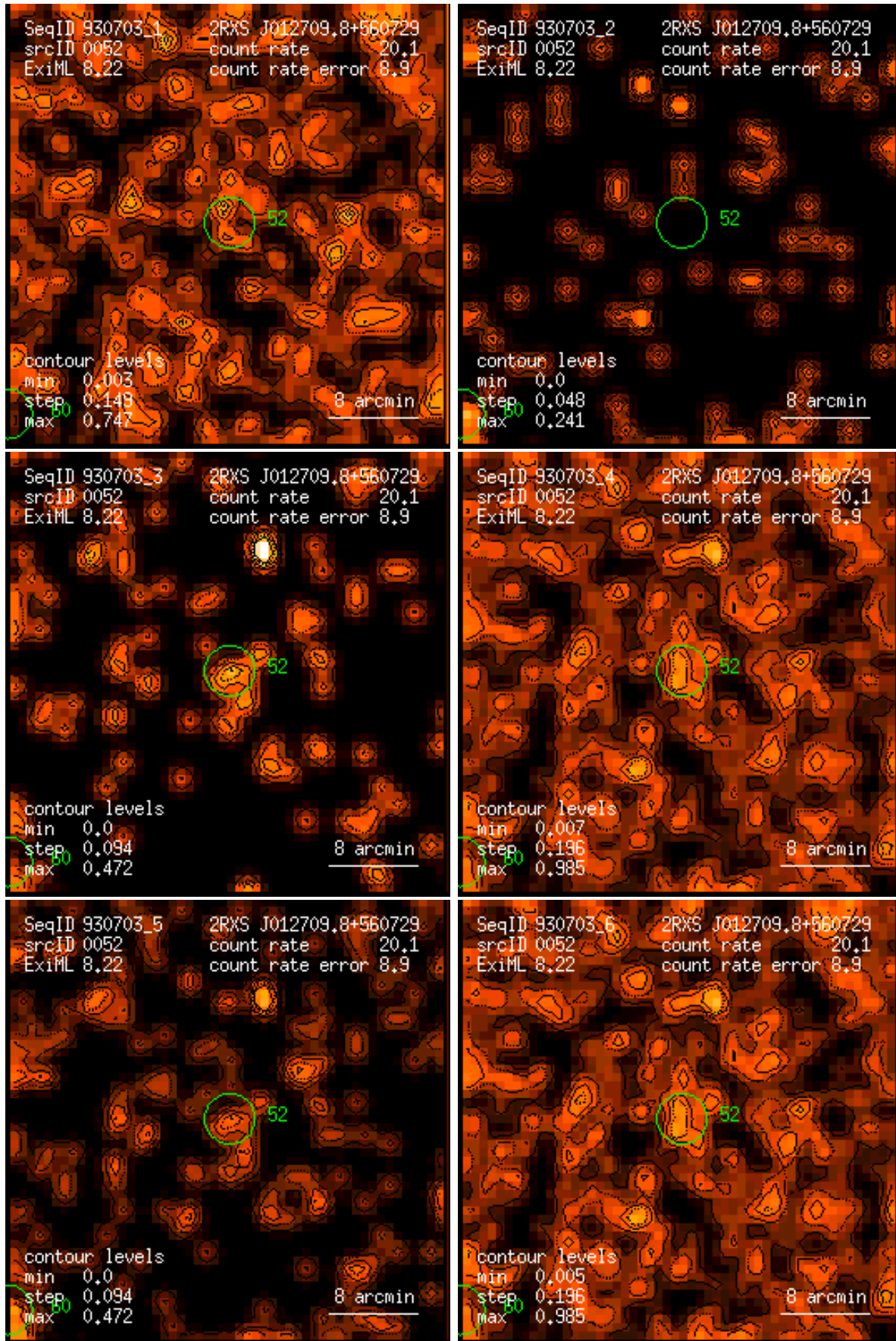
Figure 52: RASS 930703: detection 0052: band rate images, Gaussian filter: (1) PSPC channels 11 – 41, (2) 52 – 90, (3) 91 – 201, (4) 11 – 235, (5) 52 – 201, (6) 11 – 201. Broad band rates in counts/ks. Band rate contour levels in counts/ks/arcmin 2 .
