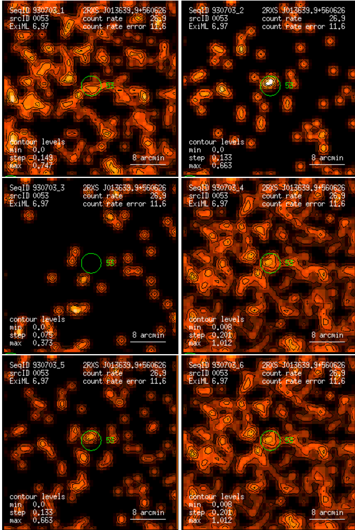
Figure 53: RASS 930703: detection 0053: band rate images, Gaussian filter: (1) PSPC channels 11 – 41, (2) 52 – 90, (3) 91 – 201, (4) 11 – 235, (5) 52 – 201, (6) 11 – 201. Broad band rates in counts/ks. Band rate contour levels in counts/ks/arcmin 2 .
