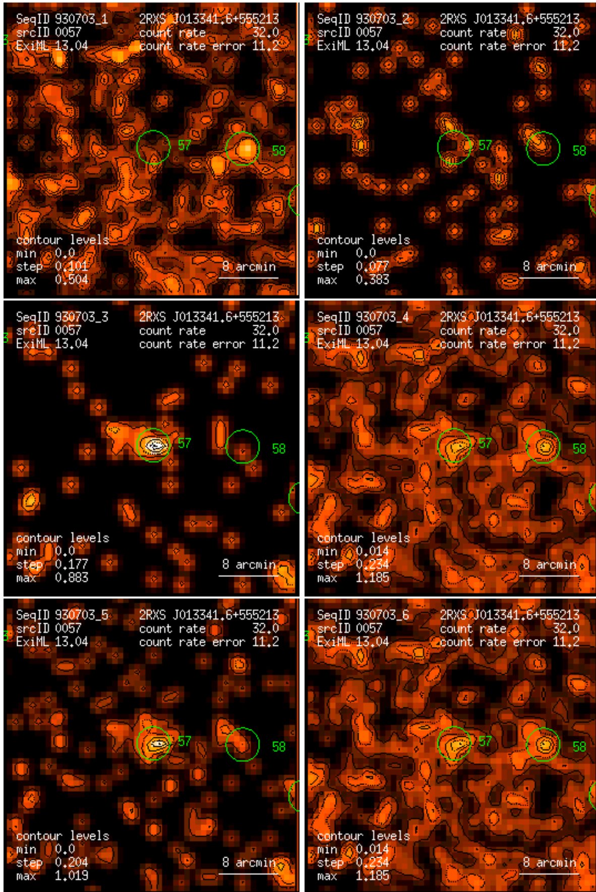
Figure 57: RASS 930703: detection 0057: band rate images, Gaussian filter: (1) PSPC channels 11 – 41, (2) 52 – 90, (3) 91 – 201, (4) 11 – 235, (5) 52 – 201, (6) 11 – 201. Broad band rates in counts/ks. Band rate contour levels in counts/ks/arcmin 2 .
