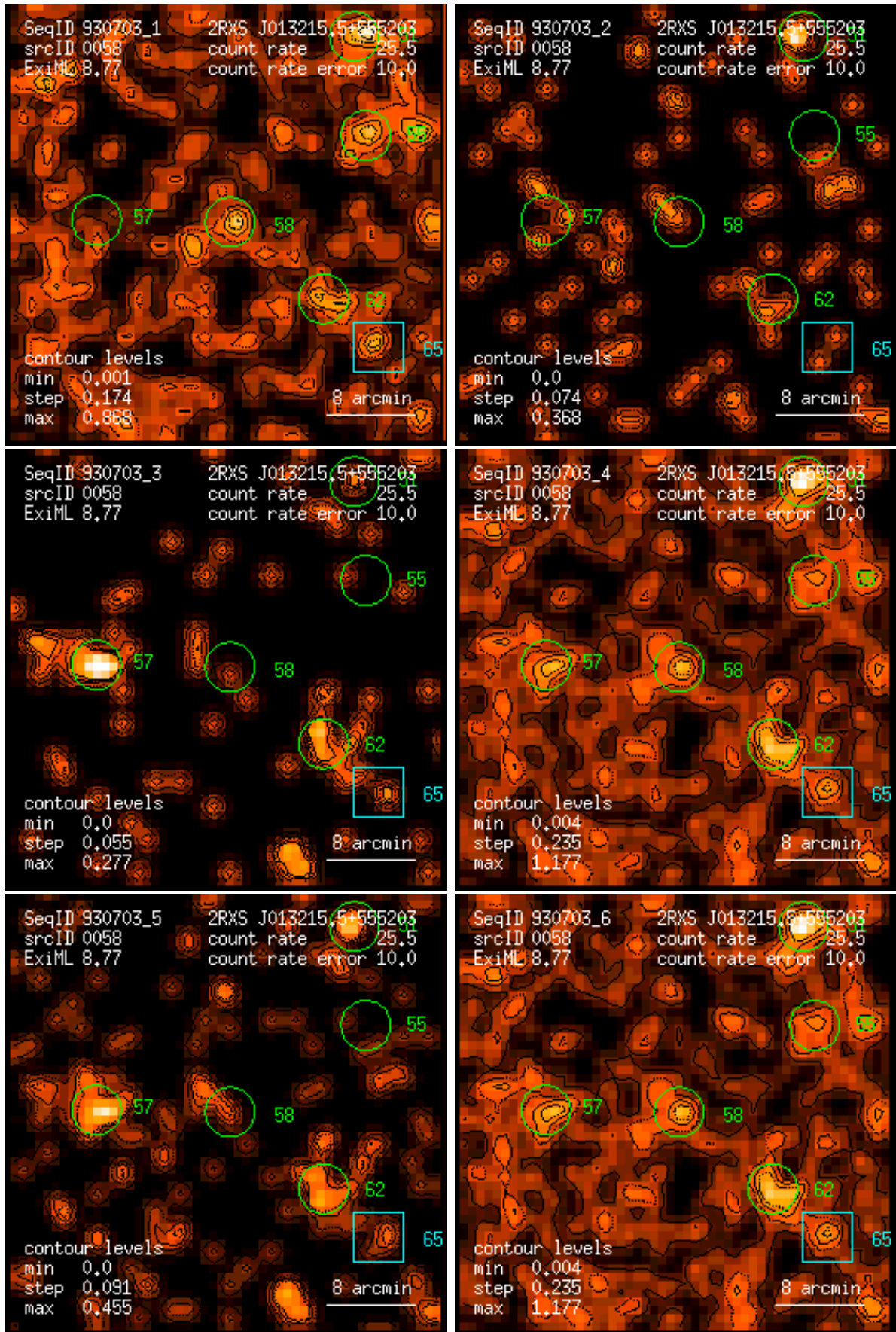
Figure 58: RASS 930703: detection 0058: band rate images, Gaussian filter: (1) PSPC channels 11 – 41, (2) 52 – 90, (3) 91 – 201, (4) 11 – 235, (5) 52 – 201, (6) 11 – 201. Broad band rates in counts/ks. Band rate contour levels in counts/ks/arcmin 2 .
