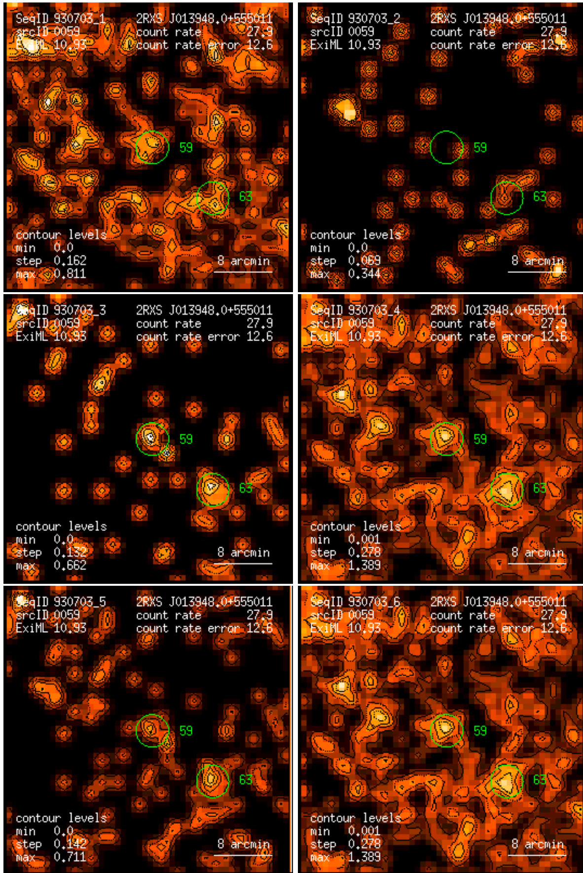
Figure 59: RASS 930703: detection 0059: band rate images, Gaussian filter: (1) PSPC channels 11 – 41, (2) 52 – 90, (3) 91 – 201, (4) 11 – 235, (5) 52 – 201, (6) 11 – 201. Broad band rates in counts/ks. Band rate contour levels in counts/ks/arcmin 2 .
