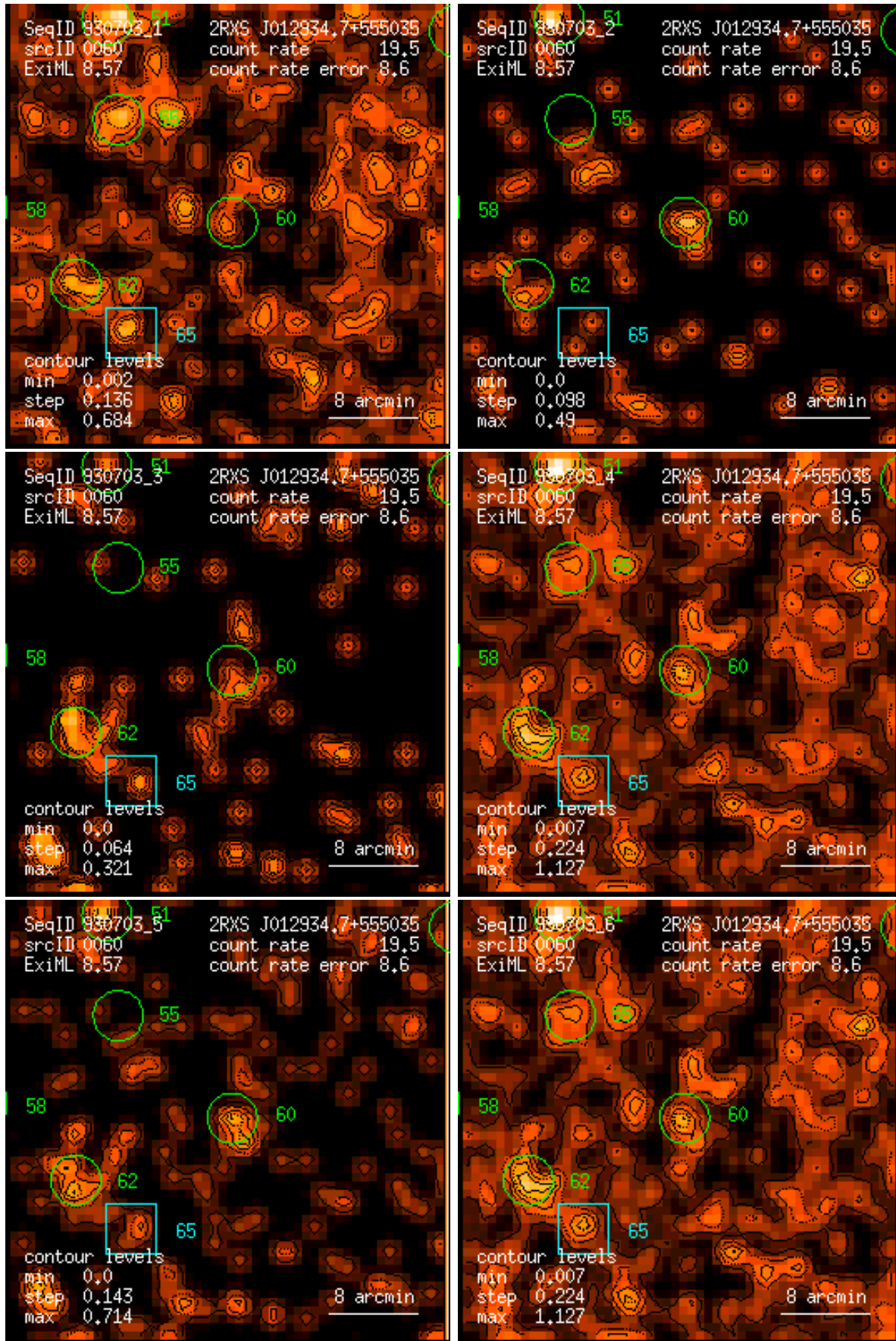
Figure 60: RASS 930703: detection 0060: band rate images, Gaussian filter: (1) PSPC channels 11 – 41, (2) 52 – 90, (3) 91 – 201, (4) 11 – 235, (5) 52 – 201, (6) 11 – 201. Broad band rates in counts/ks. Band rate contour levels in counts/ks/arcmin 2 .
