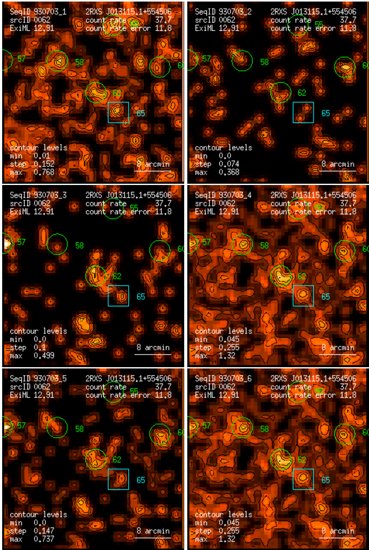
Figure 62: RASS 930703: detection 0062: band rate images, Gaussian filter: (1) PSPC channels 11 – 41, (2) 52 – 90, (3) 91 – 201, (4) 11 – 235, (5) 52 – 201, (6) 11 – 201. Broad band rates in counts/ks. Band rate contour levels in counts/ks/arcmin 2 .
