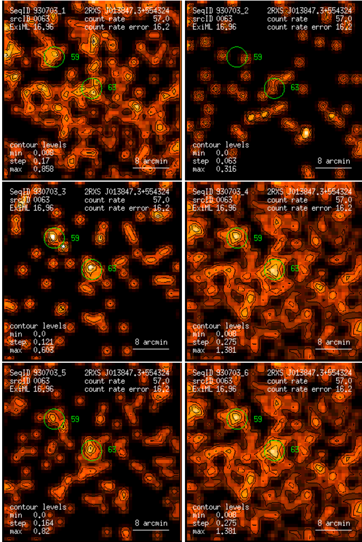
Figure 63: RASS 930703: detection 0063: band rate images, Gaussian filter: (1) PSPC channels 11 – 41, (2) 52 – 90, (3) 91 – 201, (4) 11 – 235, (5) 52 – 201, (6) 11 – 201. Broad band rates in counts/ks. Band rate contour levels in counts/ks/arcmin 2 .
