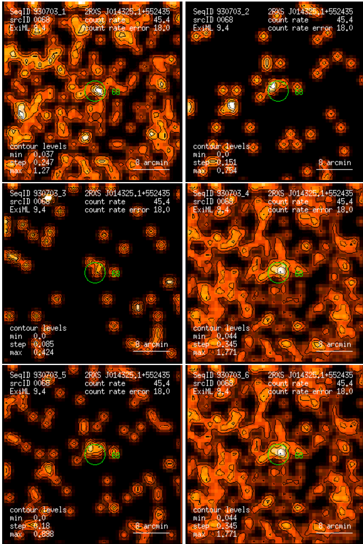
Figure 68: RASS 930703: detection 0068: band rate images, Gaussian filter: (1) PSPC channels 11 – 41, (2) 52 – 90, (3) 91 – 201, (4) 11 – 235, (5) 52 – 201, (6) 11 – 201. Broad band rates in counts/ks. Band rate contour levels in counts/ks/arcmin 2 .
