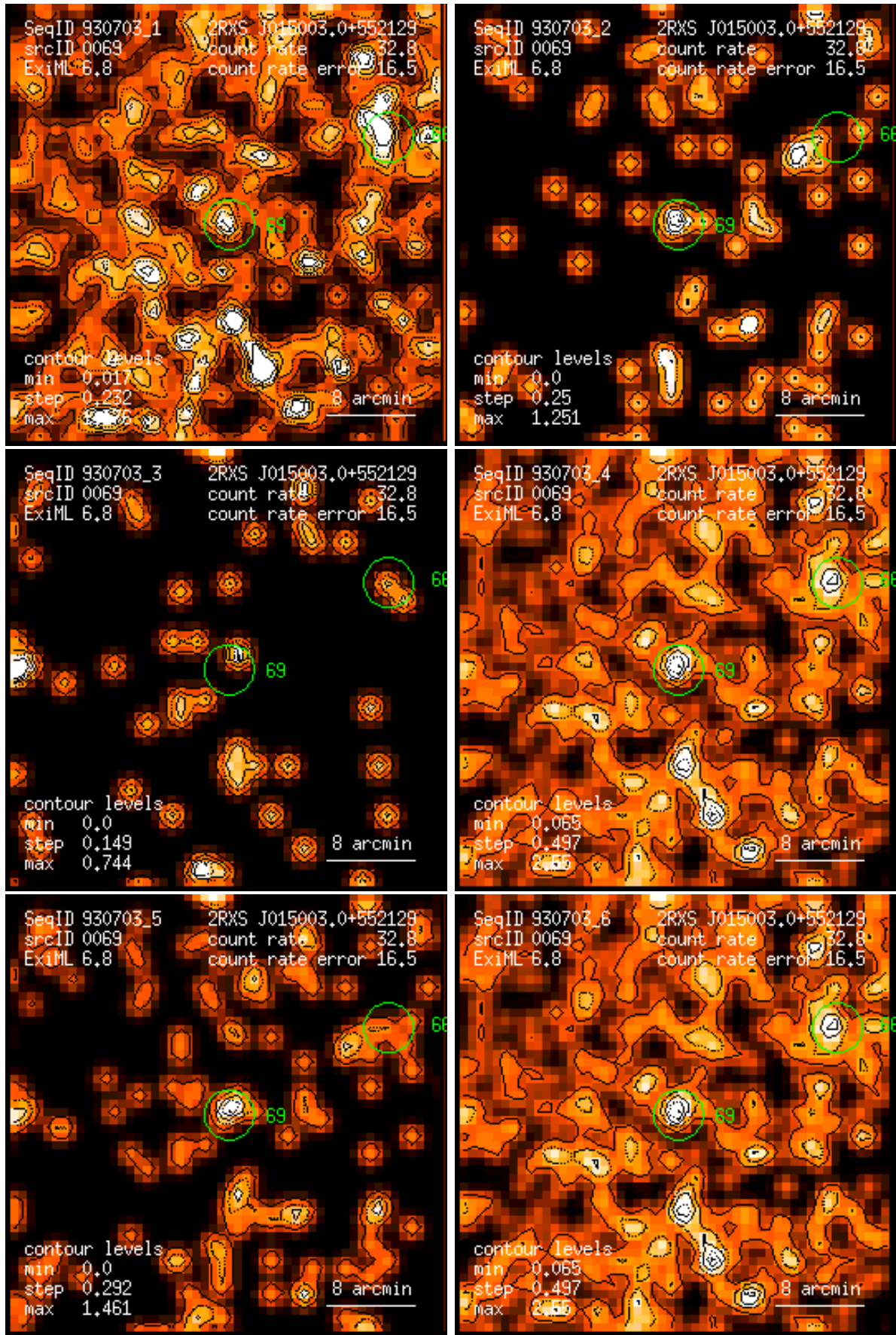
Figure 69: RASS 930703: detection 0069: band rate images, Gaussian filter: (1) PSPC channels 11 – 41, (2) 52 – 90, (3) 91 – 201, (4) 11 – 235, (5) 52 – 201, (6) 11 – 201. Broad band rates in counts/ks. Band rate contour levels in counts/ks/arcmin 2 .
