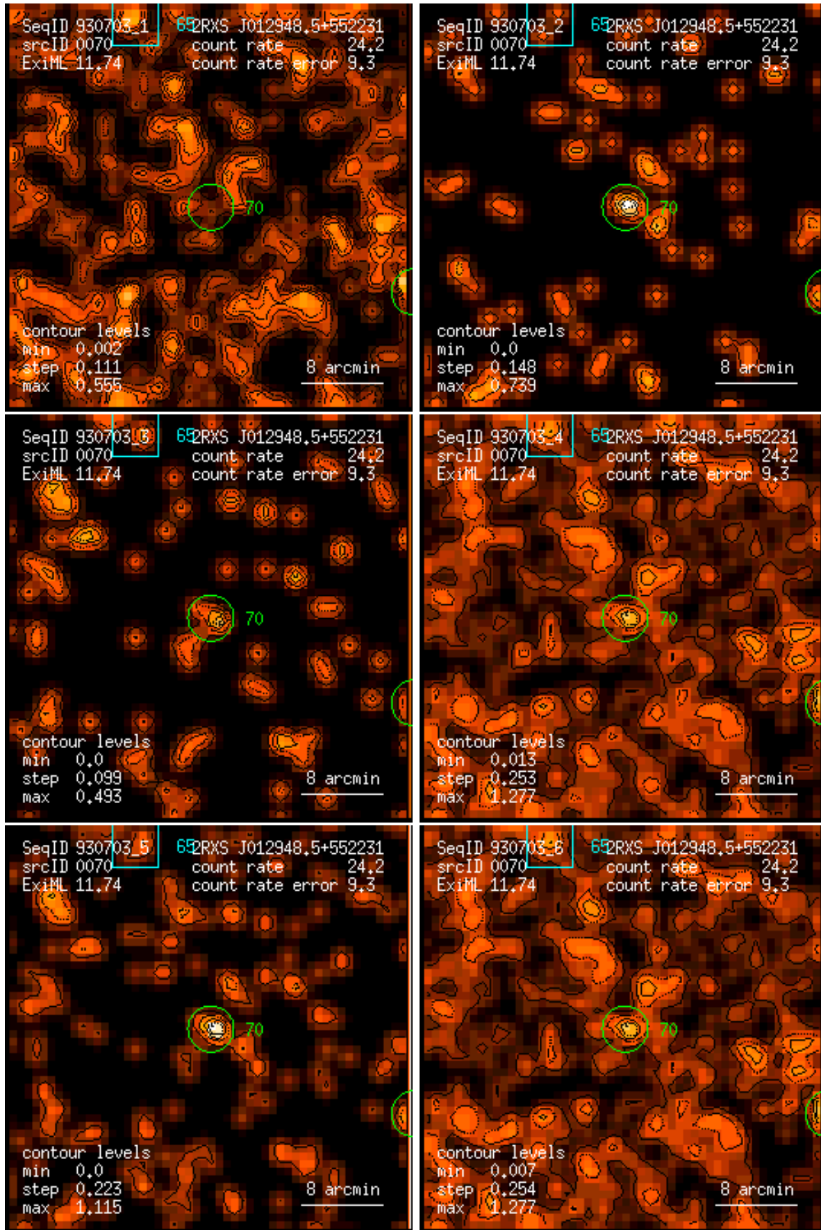
Figure 70: RASS 930703: detection 0070: band rate images, Gaussian filter: (1) PSPC channels 11 – 41, (2) 52 – 90, (3) 91 – 201, (4) 11 – 235, (5) 52 – 201, (6) 11 – 201. Broad band rates in counts/ks. Band rate contour levels in counts/ks/arcmin 2 .
