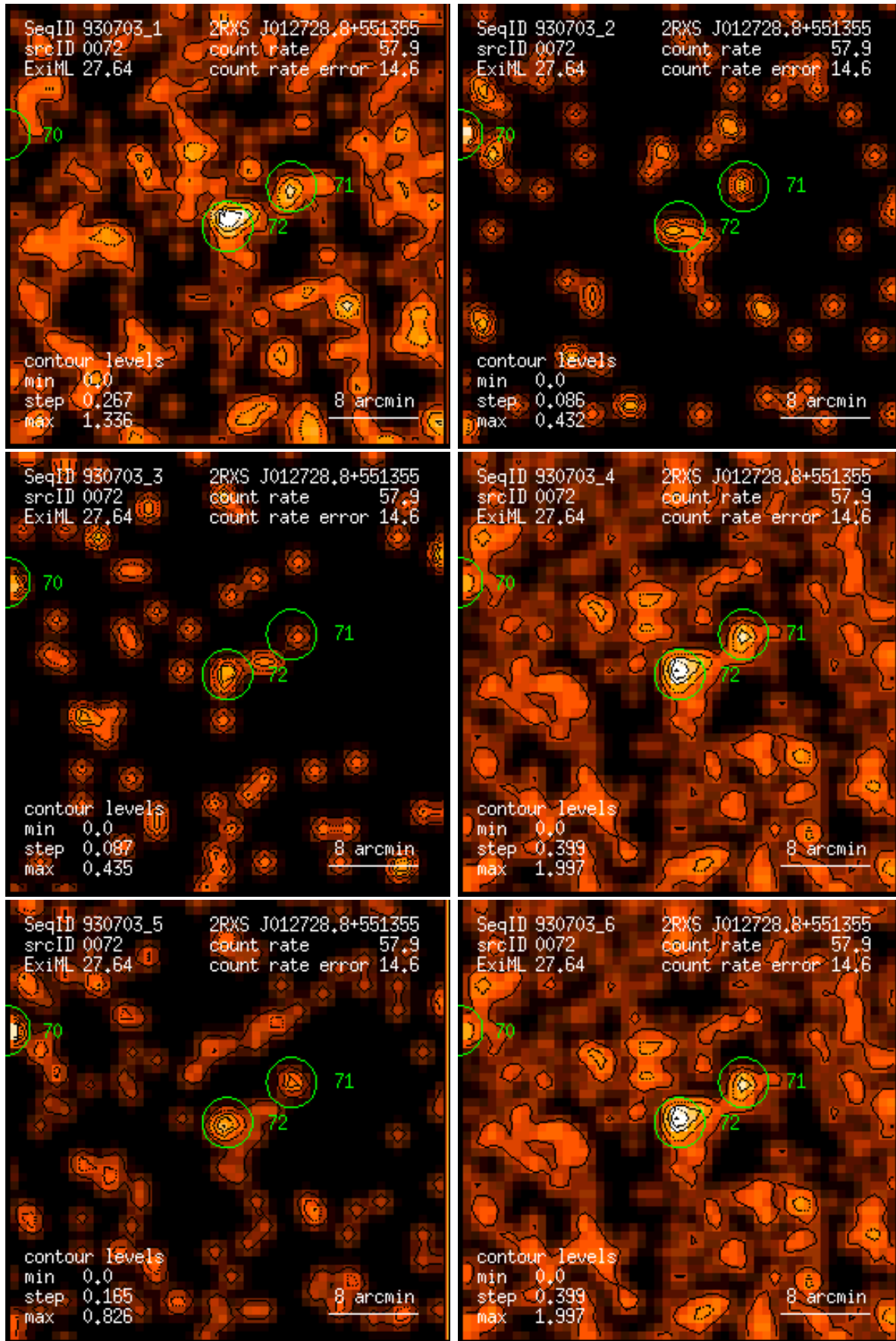
Figure 72: RASS 930703: detection 0072: band rate images, Gaussian filter: (1) PSPC channels 11 – 41, (2) 52 – 90, (3) 91 – 201, (4) 11 – 235, (5) 52 – 201, (6) 11 – 201. Broad band rates in counts/ks. Band rate contour levels in counts/ks/arcmin 2 .
