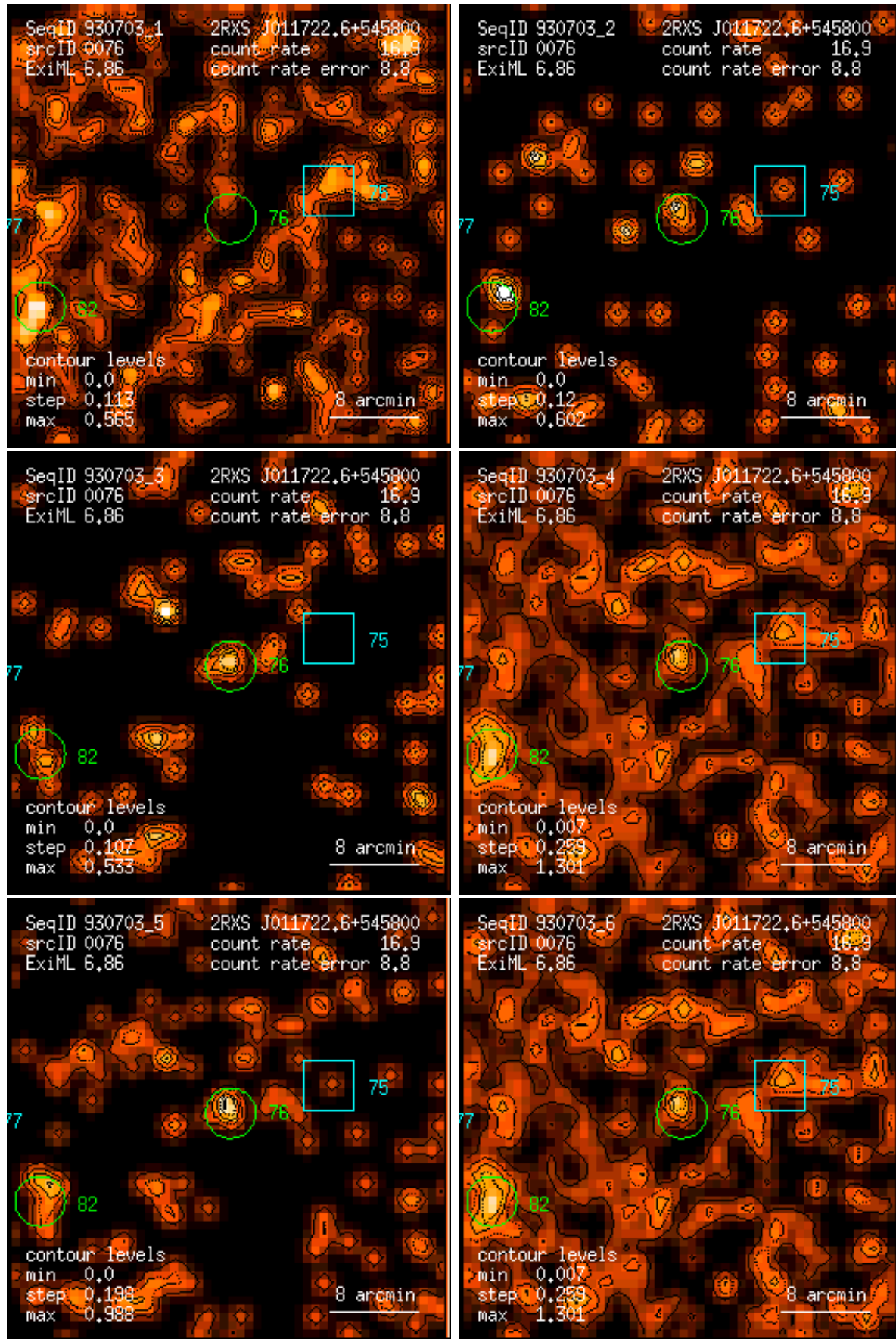
Figure 76: RASS 930703: detection 0076: band rate images, Gaussian filter: (1) PSPC channels 11 – 41, (2) 52 – 90, (3) 91 – 201, (4) 11 – 235, (5) 52 – 201, (6) 11 – 201. Broad band rates in counts/ks. Band rate contour levels in counts/ks/arcmin 2 .
