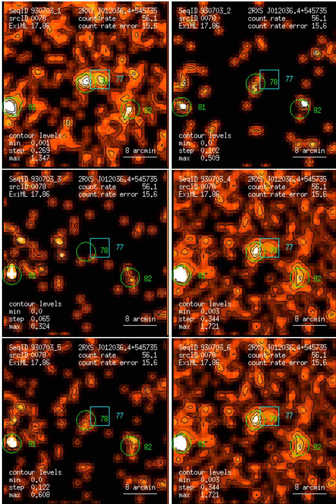
Figure 78: RASS 930703: detection 0078: band rate images, Gaussian filter: (1) PSPC channels 11 – 41, (2) 52 – 90, (3) 91 – 201, (4) 11 – 235, (5) 52 – 201, (6) 11 – 201. Broad band rates in counts/ks. Band rate contour levels in counts/ks/arcmin 2 .
