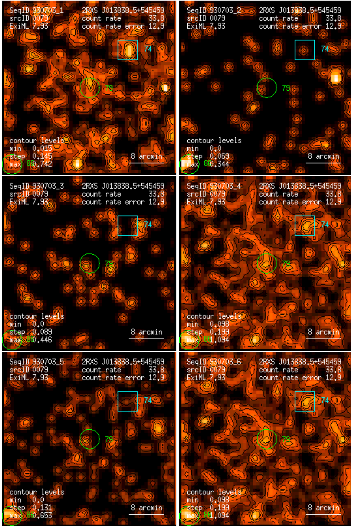
Figure 79: RASS 930703: detection 0079: band rate images, Gaussian filter: (1) PSPC channels 11 – 41, (2) 52 – 90, (3) 91 – 201, (4) 11 – 235, (5) 52 – 201, (6) 11 – 201. Broad band rates in counts/ks. Band rate contour levels in counts/ks/arcmin 2 .
