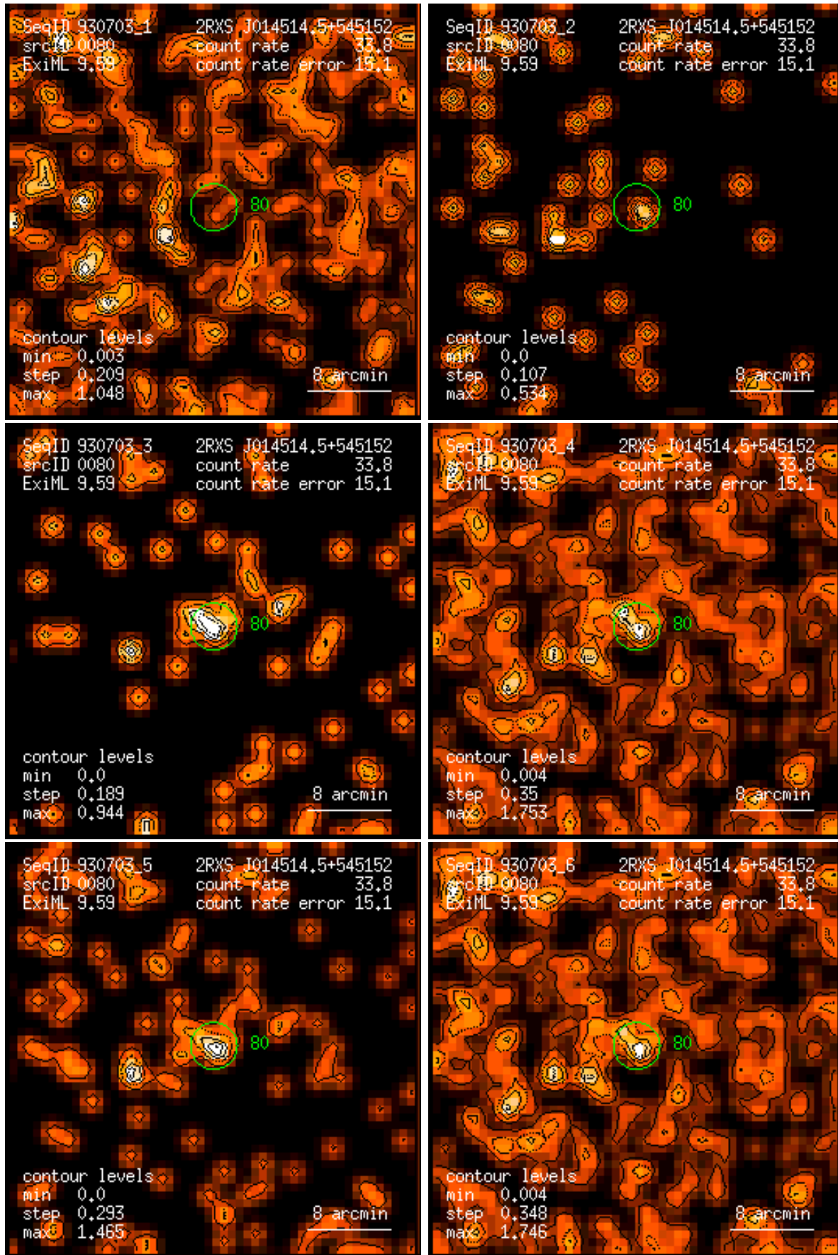
Figure 80: RASS 930703: detection 0080: band rate images, Gaussian filter: (1) PSPC channels 11 – 41, (2) 52 – 90, (3) 91 – 201, (4) 11 – 235, (5) 52 – 201, (6) 11 – 201. Broad band rates in counts/ks. Band rate contour levels in counts/ks/arcmin 2 .
