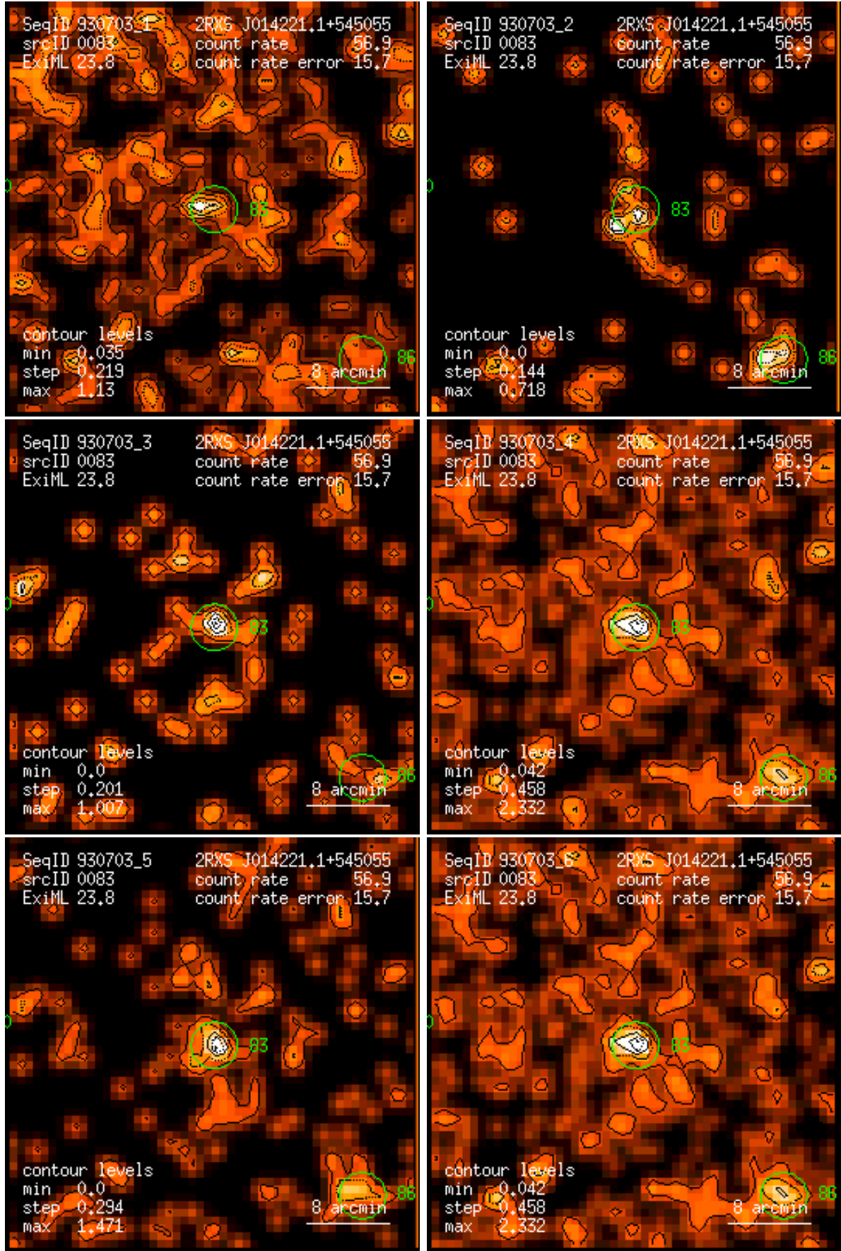
Figure 83: RASS 930703: detection 0083: band rate images, Gaussian filter: (1) PSPC channels 11 – 41, (2) 52 – 90, (3) 91 – 201, (4) 11 – 235, (5) 52 – 201, (6) 11 – 201. Broad band rates in counts/ks. Band rate contour levels in counts/ks/arcmin 2 .
