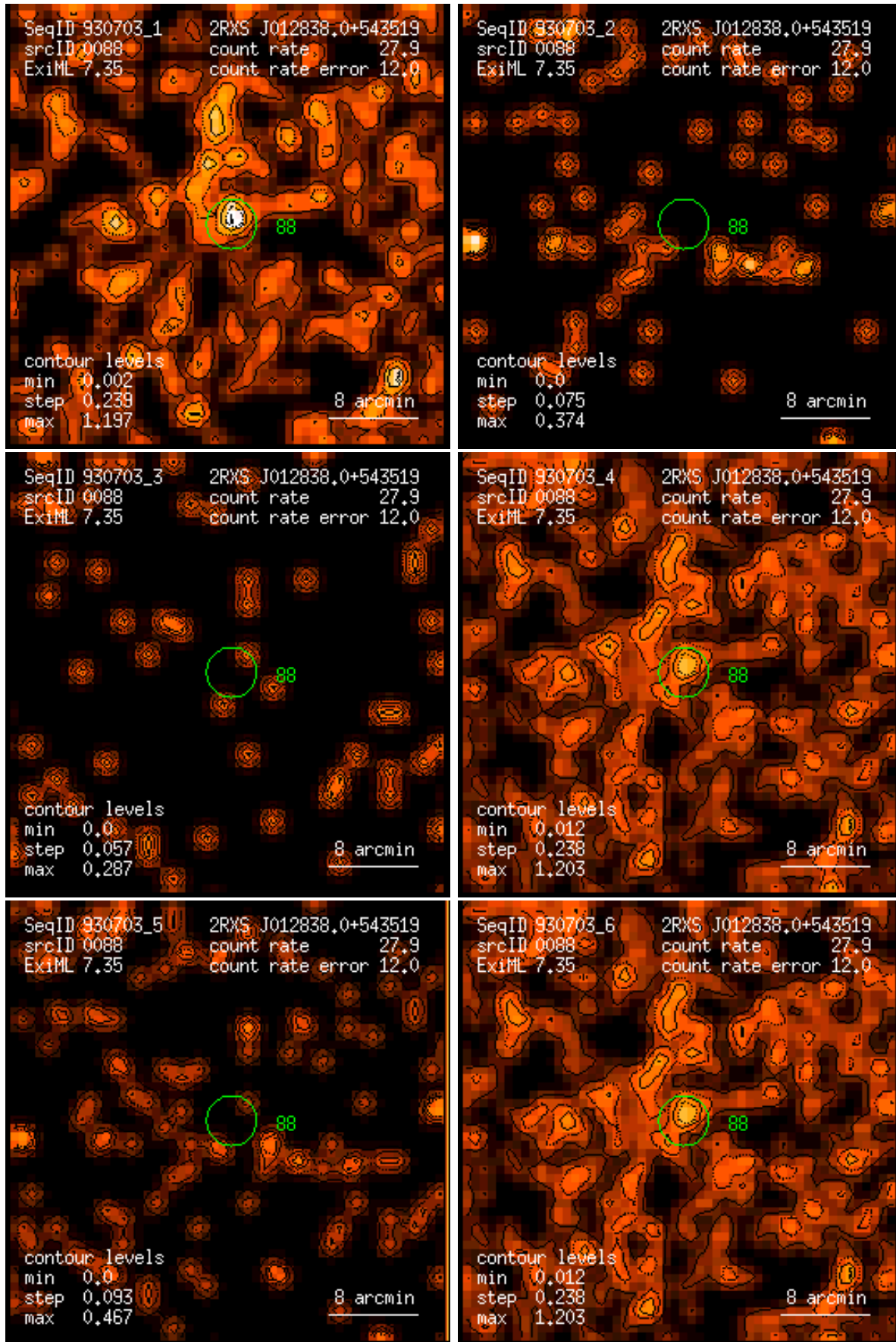
Figure 88: RASS 930703: detection 0088: band rate images, Gaussian filter: (1) PSPC channels 11 – 41, (2) 52 – 90, (3) 91 – 201, (4) 11 – 235, (5) 52 – 201, (6) 11 – 201. Broad band rates in counts/ks. Band rate contour levels in counts/ks/arcmin 2 .
