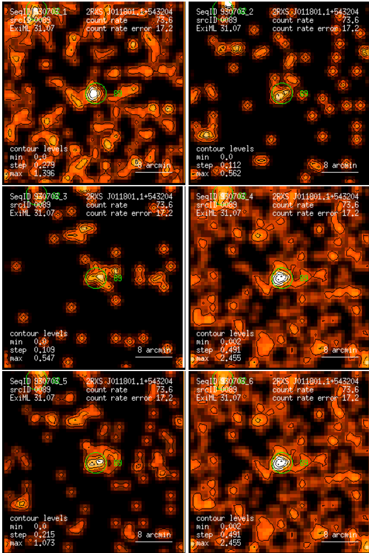
Figure 89: RASS 930703: detection 0089: band rate images, Gaussian filter: (1) PSPC channels 11 – 41, (2) 52 – 90, (3) 91 – 201, (4) 11 – 235, (5) 52 – 201, (6) 11 – 201. Broad band rates in counts/ks. Band rate contour levels in counts/ks/arcmin 2 .
