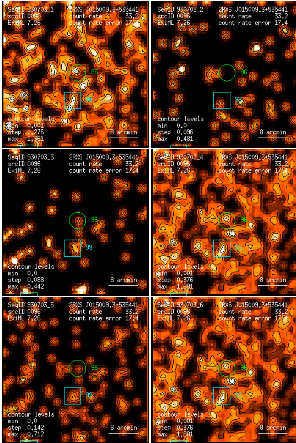
Figure 96: RASS 930703: detection 0096: band rate images, Gaussian filter: (1) PSPC channels 11 – 41, (2) 52 – 90, (3) 91 – 201, (4) 11 – 235, (5) 52 – 201, (6) 11 – 201. Broad band rates in counts/ks. Band rate contour levels in counts/ks/arcmin 2 .
