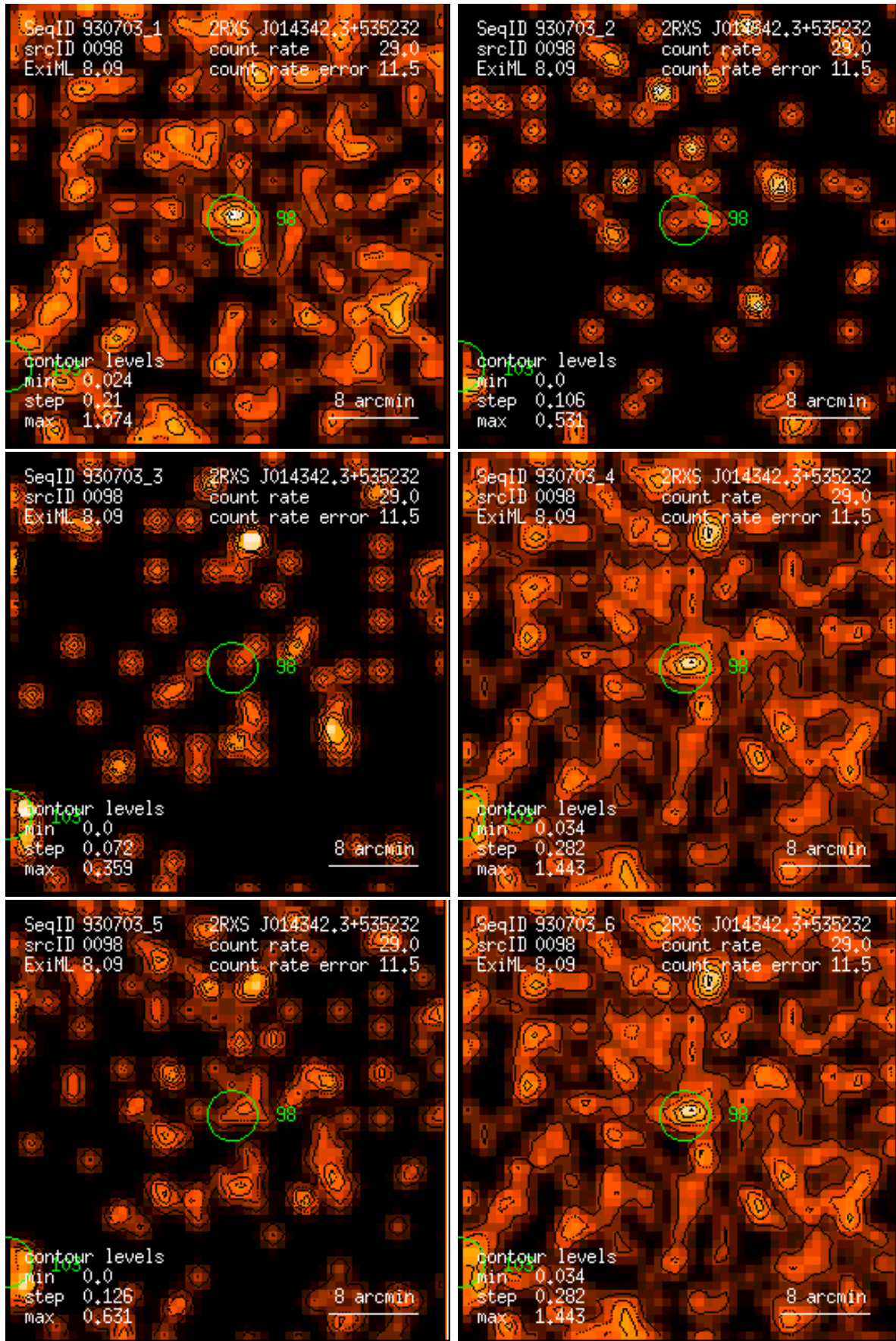
Figure 98: RASS 930703: detection 0098: band rate images, Gaussian filter: (1) PSPC channels 11 – 41, (2) 52 – 90, (3) 91 – 201, (4) 11 – 235, (5) 52 – 201, (6) 11 – 201. Broad band rates in counts/ks. Band rate contour levels in counts/ks/arcmin 2 .
