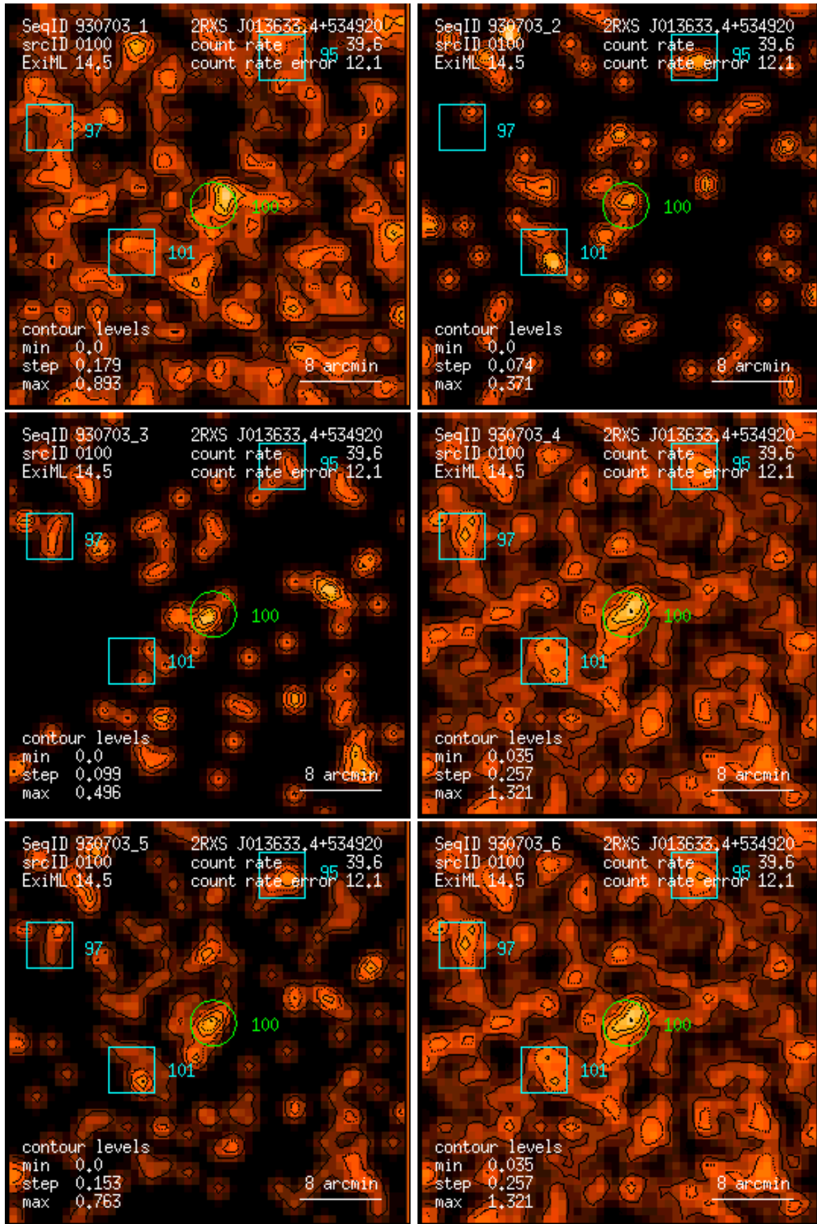
Figure 100: RASS 930703: detection 0100: band rate images, Gaussian filter: (1) PSPC channels 11 – 41, (2) 52 – 90, (3) 91 – 201, (4) 11 – 235, (5) 52 – 201, (6) 11 – 201. Broad band rates in counts/ks. Band rate contour levels in counts/ks/arcmin 2 .
