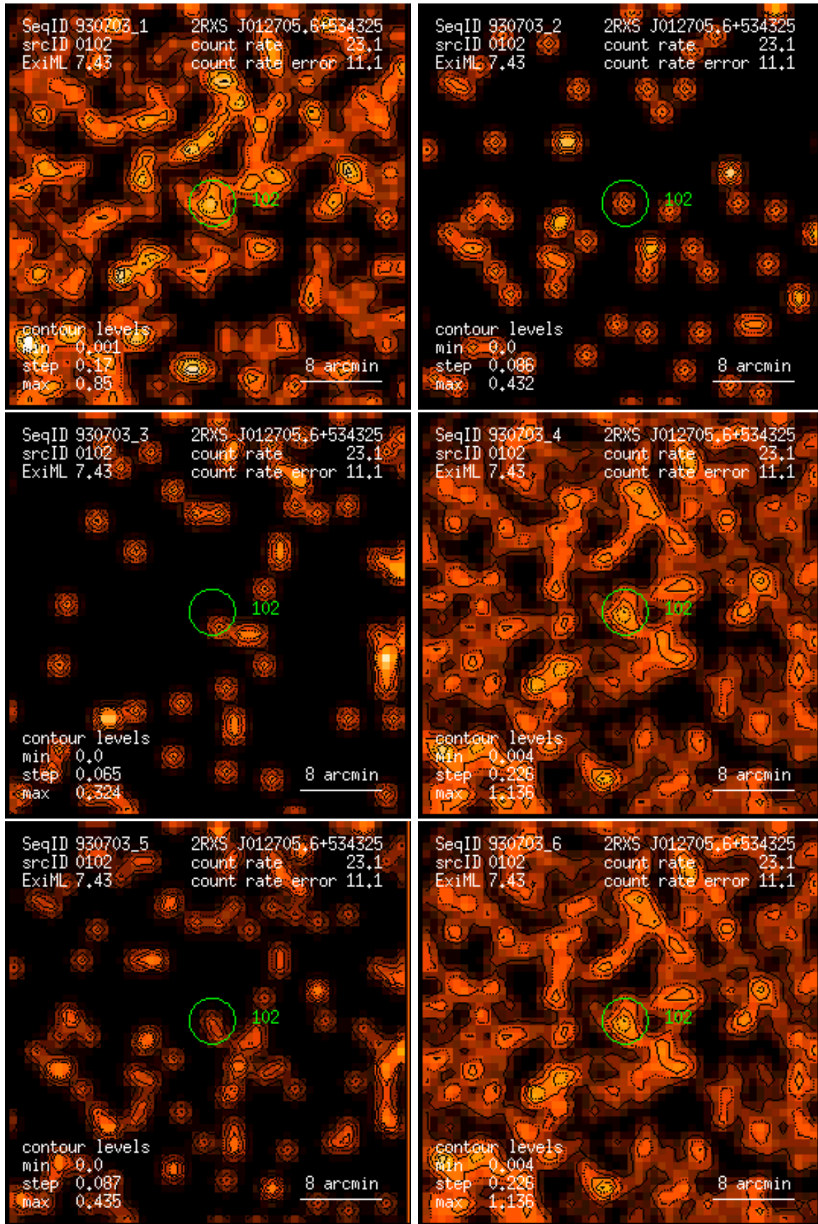
Figure 102: RASS 930703: detection 0102: band rate images, Gaussian filter: (1) PSPC channels 11 – 41, (2) 52 – 90, (3) 91 – 201, (4) 11 – 235, (5) 52 – 201, (6) 11 – 201. Broad band rates in counts/ks. Band rate contour levels in counts/ks/arcmin 2 .
