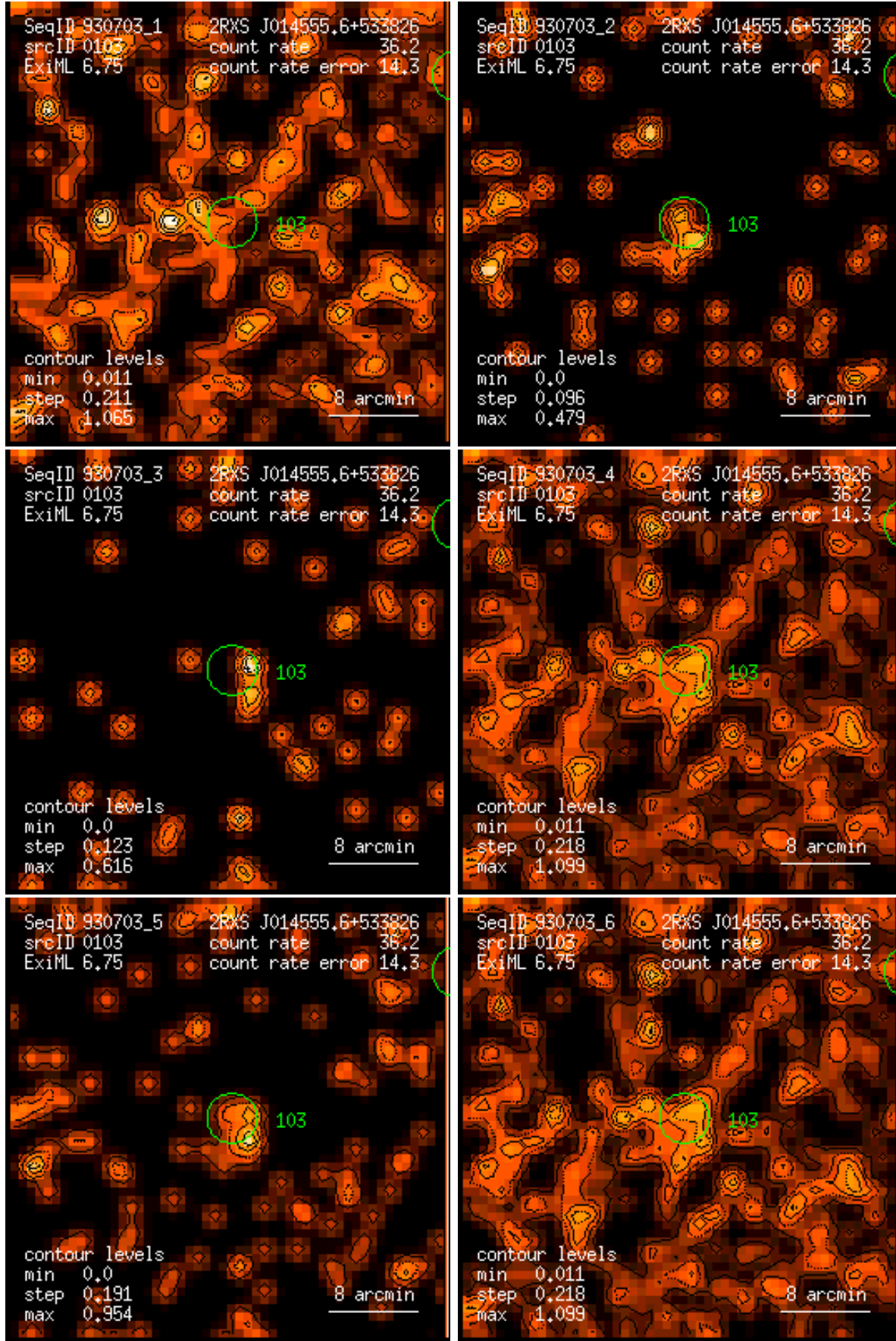
Figure 103: RASS 930703: detection 0103: band rate images, Gaussian filter: (1) PSPC channels 11 – 41, (2) 52 – 90, (3) 91 – 201, (4) 11 – 235, (5) 52 – 201, (6) 11 – 201. Broad band rates in counts/ks. Band rate contour levels in counts/ks/arcmin 2 .
