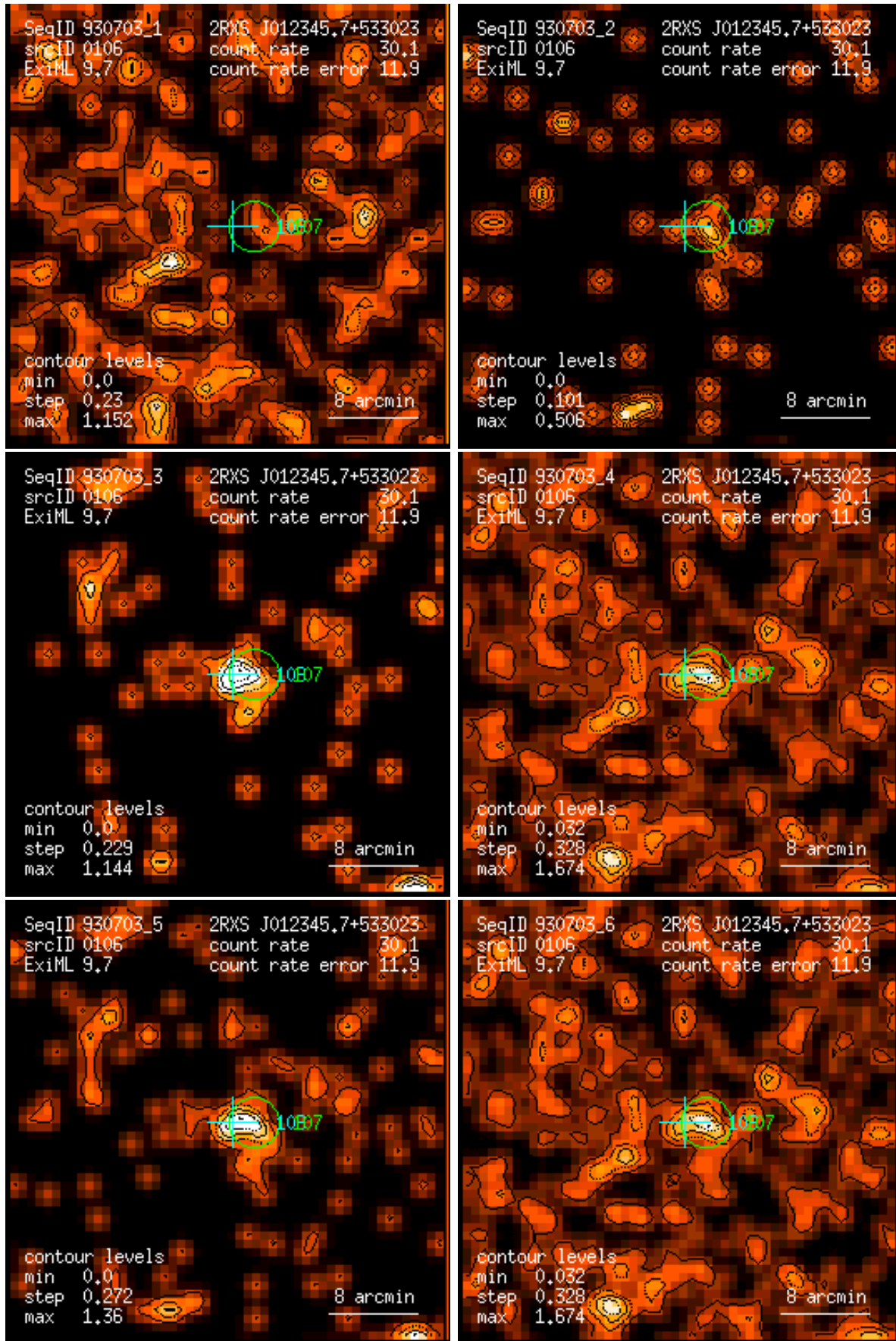
Figure 106: RASS 930703: detection 0106: band rate images, Gaussian filter: (1) PSPC channels 11 – 41, (2) 52 – 90, (3) 91 – 201, (4) 11 – 235, (5) 52 – 201, (6) 11 – 201. Broad band rates in counts/ks. Band rate contour levels in counts/ks/arcmin 2 .
