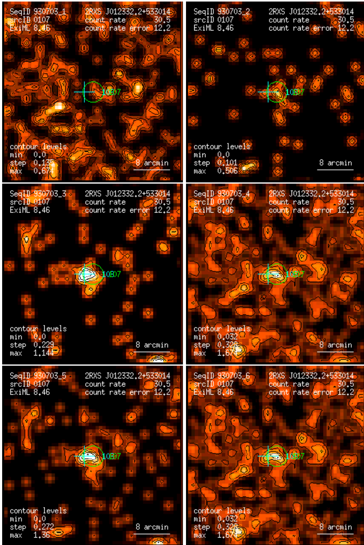
Figure 107: RASS 930703: detection 0107: band rate images, Gaussian filter: (1) PSPC channels 11 – 41, (2) 52 – 90, (3) 91 – 201, (4) 11 – 235, (5) 52 – 201, (6) 11 – 201. Broad band rates in counts/ks. Band rate contour levels in counts/ks/arcmin 2 .
