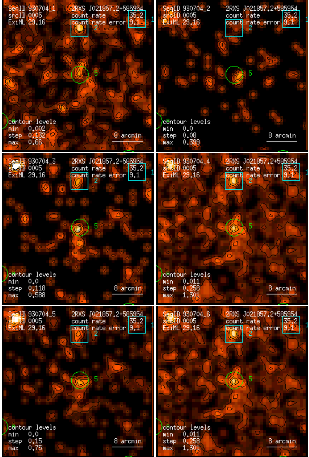
Figure 5: RASS 930704: detection 0005: band rate images, Gaussian filter: (1) PSPC channels 11 – 41, (2) 52 – 90, (3) 91 – 201, (4) 11 – 235, (5) 52 – 201, (6) 11 – 201. Broad band rates in counts/ks. Band rate contour levels in counts/ks/arcmin 2 .
