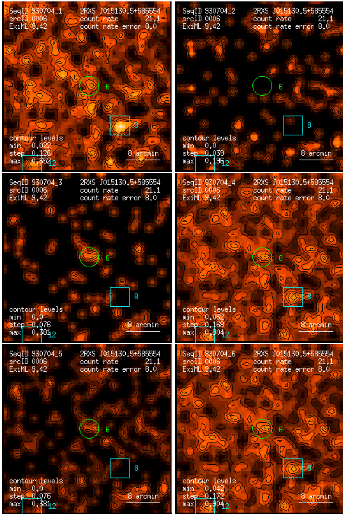
Figure 6: RASS 930704: detection 0006: band rate images, Gaussian filter: (1) PSPC channels 11 – 41, (2) 52 – 90, (3) 91 – 201, (4) 11 – 235, (5) 52 – 201, (6) 11 – 201. Broad band rates in counts/ks. Band rate contour levels in counts/ks/arcmin 2 .
