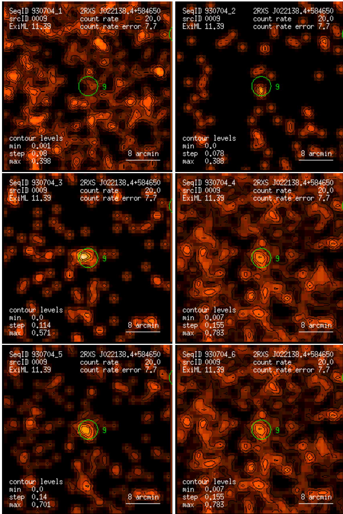
Figure 9: RASS 930704: detection 0009: band rate images, Gaussian filter: (1) PSPC channels 11 – 41, (2) 52 – 90, (3) 91 – 201, (4) 11 – 235, (5) 52 – 201, (6) 11 – 201. Broad band rates in counts/ks. Band rate contour levels in counts/ks/arcmin 2 .
