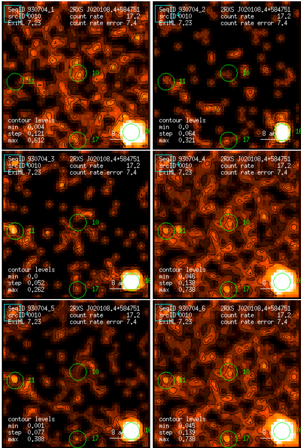
Figure 10: RASS 930704: detection 0010: band rate images, Gaussian filter: (1) PSPC channels 11 – 41, (2) 52 – 90, (3) 91 – 201, (4) 11 – 235, (5) 52 – 201, (6) 11 – 201. Broad band rates in counts/ks. Band rate contour levels in counts/ks/arcmin 2 .
