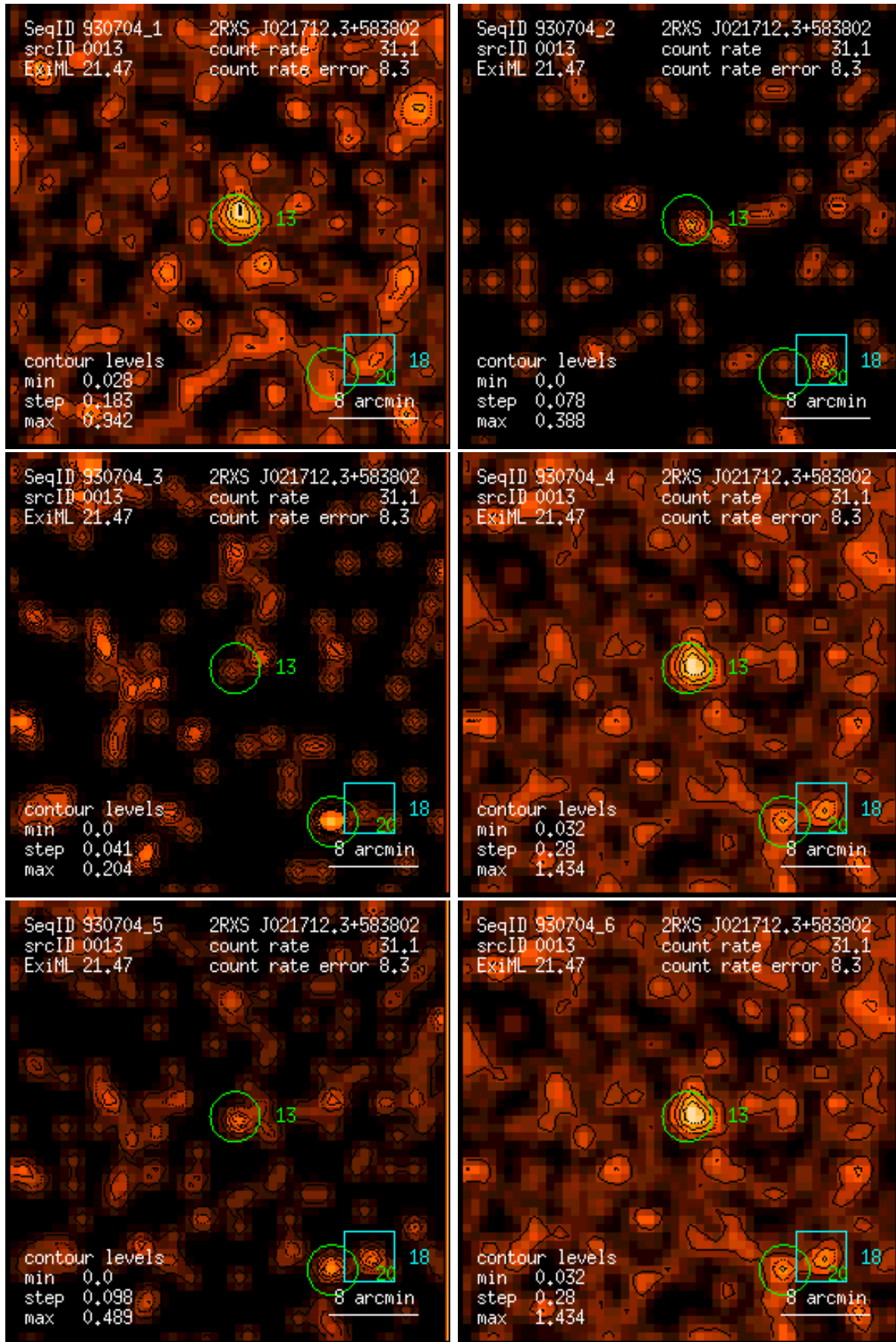
Figure 13: RASS 930704: detection 0013: band rate images, Gaussian filter: (1) PSPC channels 11 – 41, (2) 52 – 90, (3) 91 – 201, (4) 11 – 235, (5) 52 – 201, (6) 11 – 201. Broad band rates in counts/ks. Band rate contour levels in counts/ks/arcmin 2 .
