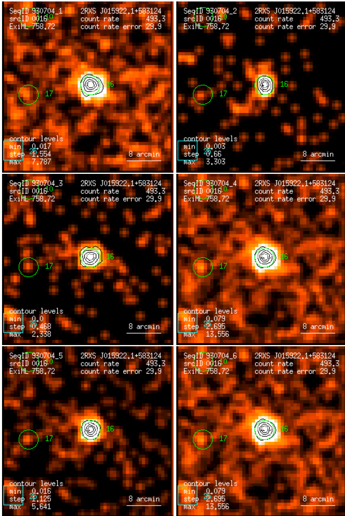
Figure 16: RASS 930704: detection 0016: band rate images, Gaussian filter: (1) PSPC channels 11 – 41, (2) 52 – 90, (3) 91 – 201, (4) 11 – 235, (5) 52 – 201, (6) 11 – 201. Broad band rates in counts/ks. Band rate contour levels in counts/ks/arcmin 2 .
