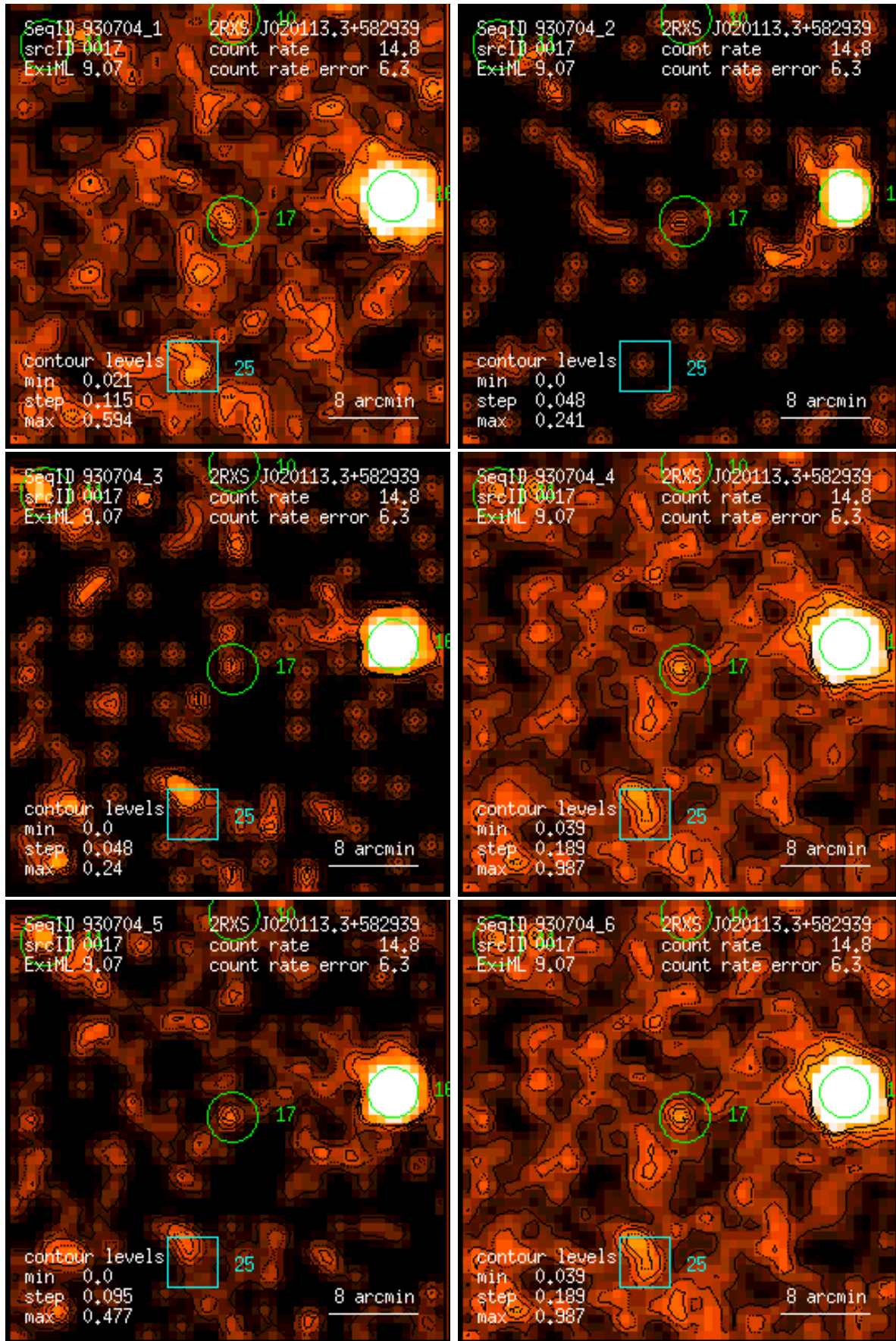
Figure 17: RASS 930704: detection 0017: band rate images, Gaussian filter: (1) PSPC channels 11 – 41, (2) 52 – 90, (3) 91 – 201, (4) 11 – 235, (5) 52 – 201, (6) 11 – 201. Broad band rates in counts/ks. Band rate contour levels in counts/ks/arcmin 2 .
