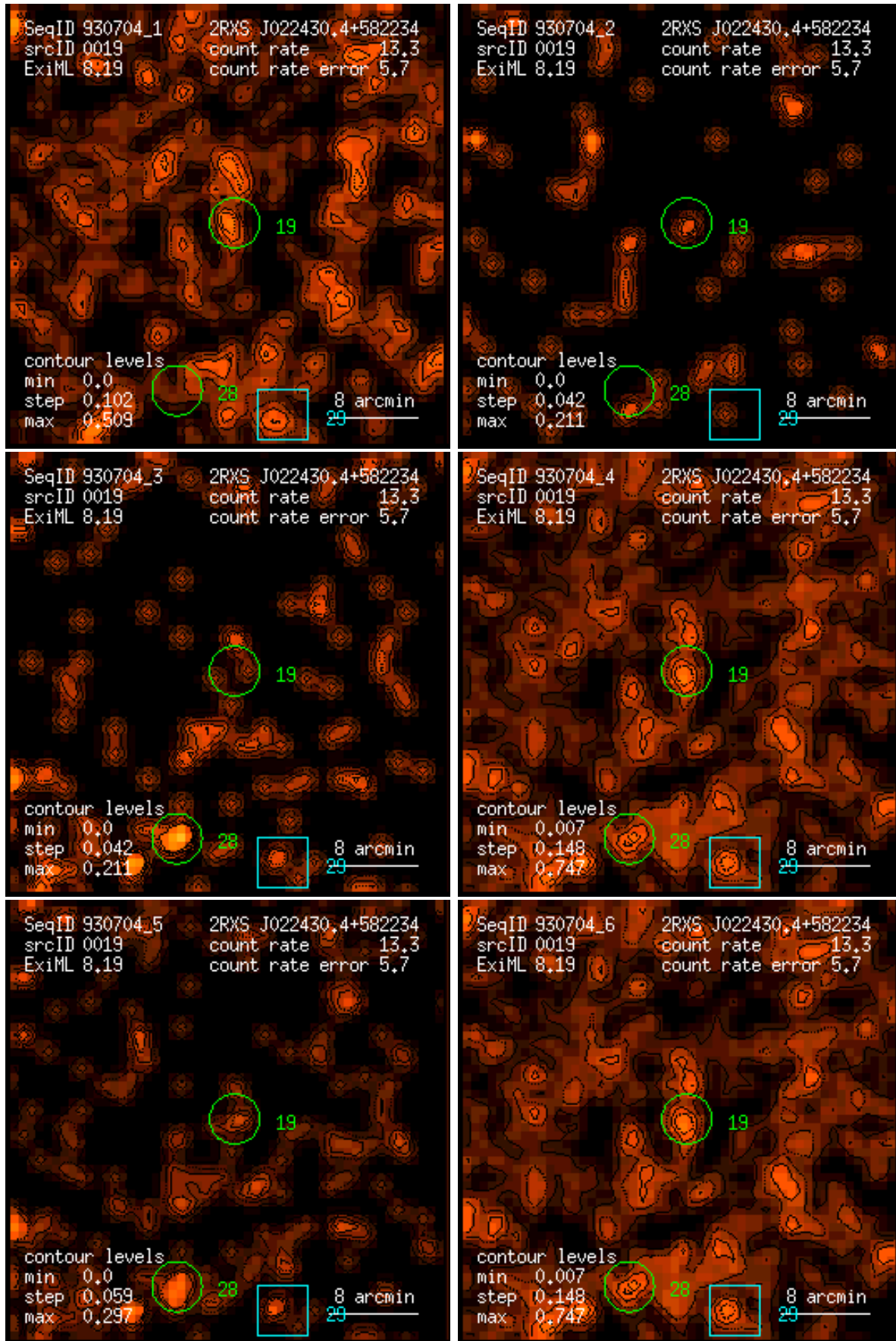
Figure 19: RASS 930704: detection 0019: band rate images, Gaussian filter: (1) PSPC channels 11 – 41, (2) 52 – 90, (3) 91 – 201, (4) 11 – 235, (5) 52 – 201, (6) 11 – 201. Broad band rates in counts/ks. Band rate contour levels in counts/ks/arcmin 2 .
