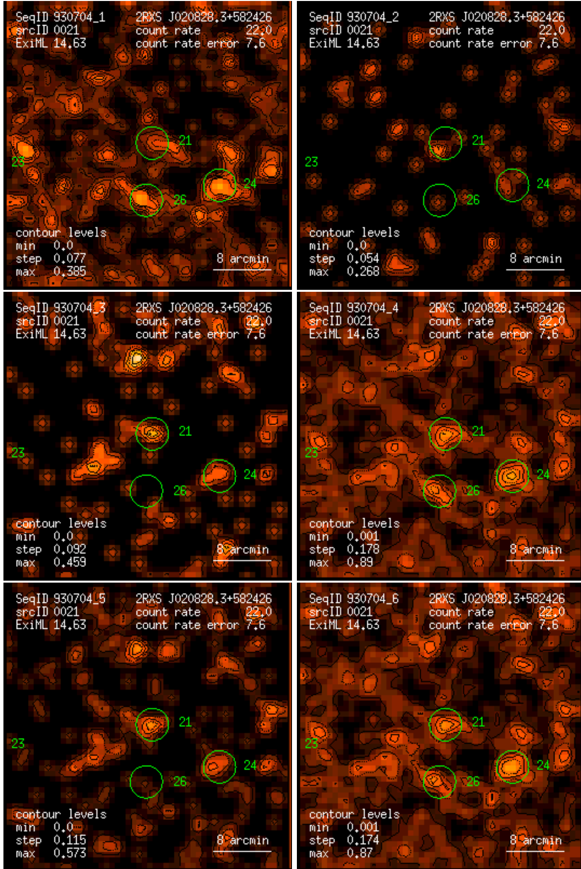
Figure 21: RASS 930704: detection 0021: band rate images, Gaussian filter: (1) PSPC channels 11 – 41, (2) 52 – 90, (3) 91 – 201, (4) 11 – 235, (5) 52 – 201, (6) 11 – 201. Broad band rates in counts/ks. Band rate contour levels in counts/ks/arcmin 2 .
