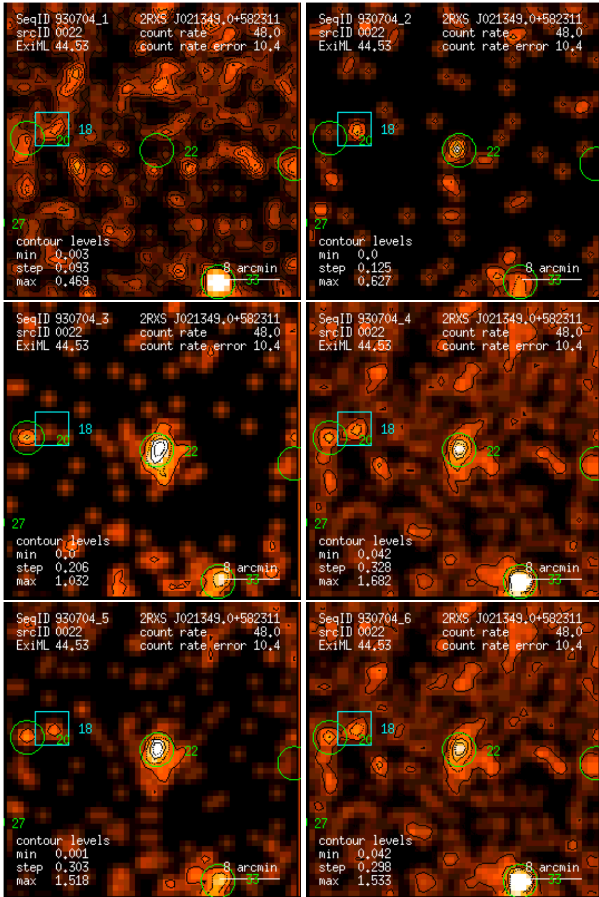
Figure 22: RASS 930704: detection 0022: band rate images, Gaussian filter: (1) PSPC channels 11 – 41, (2) 52 – 90, (3) 91 – 201, (4) 11 – 235, (5) 52 – 201, (6) 11 – 201. Broad band rates in counts/ks. Band rate contour levels in counts/ks/arcmin 2 .
